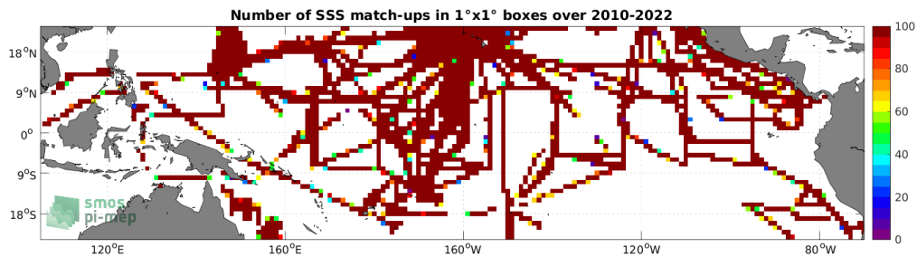
Figure 4: Number of SSS match-ups between TSG (SAMOS) SSS and the SMOS SSS L3 v332 - 9 Days (CATDS-CPDC) SSS product for the Tropical Pacific Ocean Pi-MEP region over 1^\circ \times 1^\circ boxes and for the full satellite product period.
