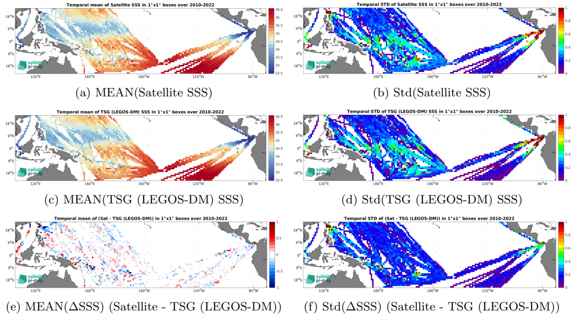
Figure 7: Temporal mean (left) and Std (right) of SSS from SMOS SSS L3 v332 - 9 Days (CATDS-CPDC) (top), TSG (LEGOS-DM) (middle), and of \Delta SSS (Satellite - TSG (LEGOS-DM)). Only match-up pairs are used to generate these maps.
