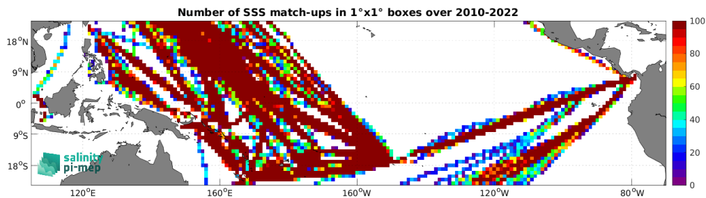
Figure 5: Number of SSS match-ups between TSG (LEGOS-DM) SSS and the SMOS SSS L3 v332 - 9 Days (CATDS-CPDC) SSS product for the Tropical Pacific Ocean Pi-MEP region over 1^\circ \times 1^\circ boxes and for the full satellite product period.
