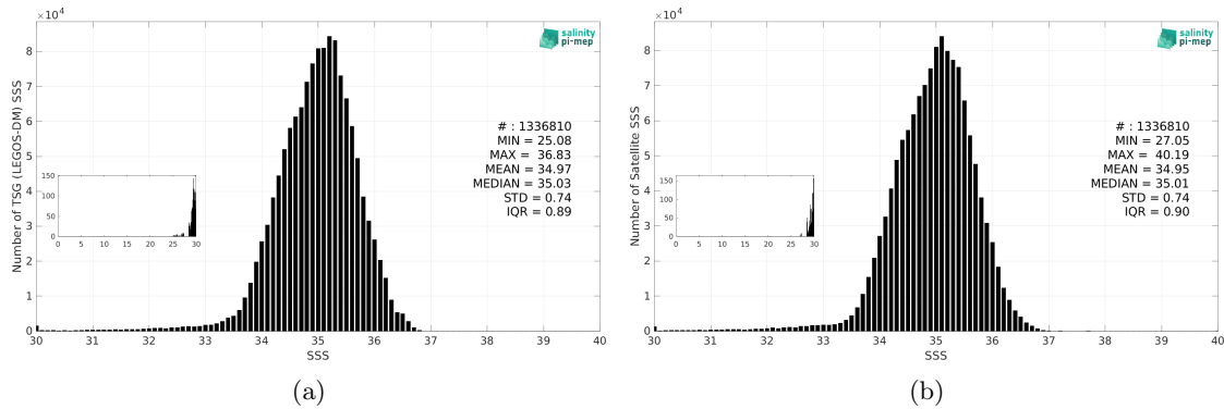
Figure 3: Histograms of SSS from TSG (LEGOS-DM) (a) and SMOS SSS L3 v332 - 9 Days (CATDS-CPDC) (b) considering all match-up pairs per bins of 0.1 over the Tropical Pacific Ocean Pi-MEP region and for the full satellite product period.
