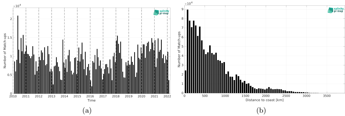
Figure 2: Number of match-ups between TSG (LEGOS-DM) and SMOS SSS L3 v332 - 9 Days (CATDS-CPDC) SSS as a function of time (a) and as function of the distance to coast (b) over the Tropical Pacific Ocean Pi-MEP region and for the full satellite product period.
