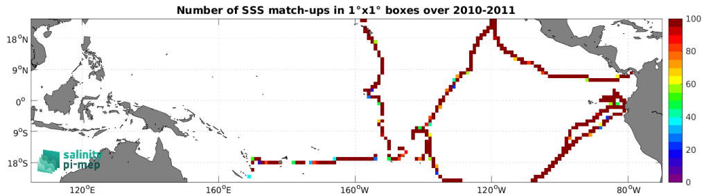
Figure 5: Number of SSS match-ups between TSG (GOSUD-Sailing-ship) SSS and the SMOS SSS L3 v332 - 9 Days (CATDS-CPDC) SSS product for the Tropical Pacific Ocean Pi-MEP region over 1^\circ \times 1^\circ boxes and for the full satellite product period.
