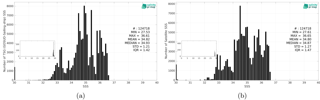
Figure 3: Histograms of SSS from TSG (GOSUD-Sailing-ship) (a) and SMOS SSS L3 v332 - 9 Days (CATDS-CPDC) (b) considering all match-up pairs per bins of 0.1 over the Tropical Pacific Ocean Pi-MEP region and for the full satellite product period.
