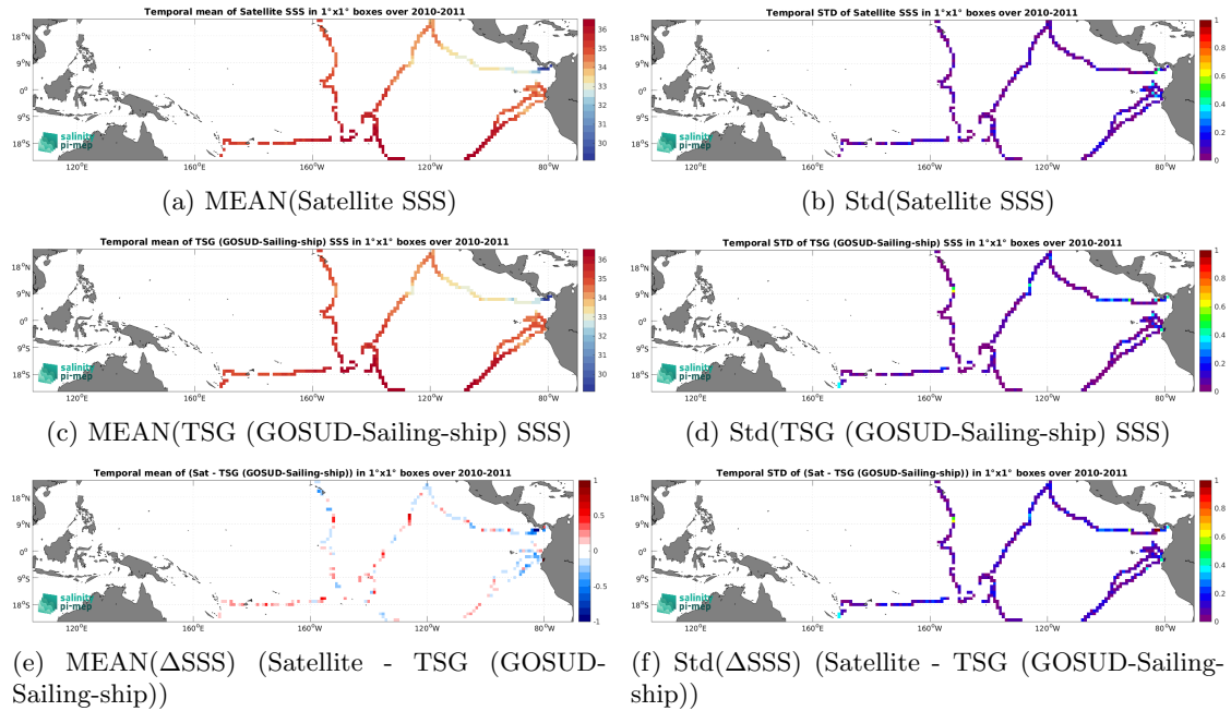
Figure 7: Temporal mean (left) and Std (right) of SSS from SMOS SSS L3 v332 - 9 Days (CATDS-CPDC) (top), TSG (GOSUD-Sailing-ship) (middle), and of \Delta SSS (Satellite - TSG (GOSUD-Sailing-ship)). Only match-up pairs are used to generate these maps.
