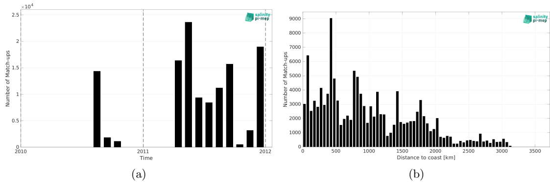
Figure 2: Number of match-ups between TSG (GOSUD-Sailing-ship) and SMOS SSS L3 v332 - 9 Days (CATDS-CPDC) SSS as a function of time (a) and as function of the distance to coast (b) over the Tropical Pacific Ocean Pi-MEP region and for the full satellite product period.
