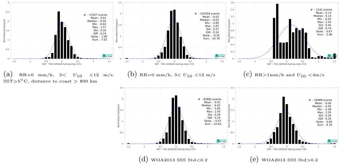
Figure 15: Normalized histogram of \Delta SSS (SMOS SSS L3 v332 - 9 Days (CATDS-CPDC) - TSG (GOSUD-Sailing-ship)) for 5 different subdatasets corresponding to: RR=0 mm/h, 3 < U_{10} < 12 m/s, SST > 5°C, distance to coast > 800 km (a), RR=0 mm/h, 3 < U_{10} < 12 m/s (b), RR > 1mm/h and U_{10} < 4 m/s (c), WOA2013 SSS Std < 0.2 (d), WOA2013 SSS Std > 0.2 (e).
