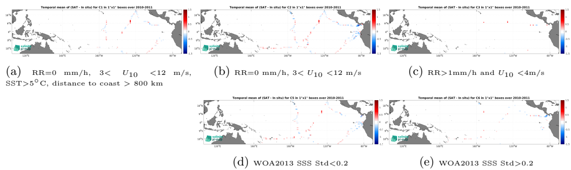
Figure 14: Temporal mean gridded over spatial boxes of size 1^\circ \times 1^\circ of \Delta SSS (SMOS SSS L3 v332 - 9 Days (CATDS-CPDC) - TSG (GOSUD-Sailing-ship)) for 5 different subdatasets corresponding to: RR=0 mm/h, 3 < U_{10} < 12 m/s, SST > 5^\circ\text{C} , distance to coast > 800 km (a), RR=0 mm/h, 3 < U_{10} < 12 m/s (b), RR > 1 mm/h and U_{10} < 4 m/s (c), WOA2013 SSS Std < 0.2 (d), WOA2013 SSS Std > 0.2 (e).
