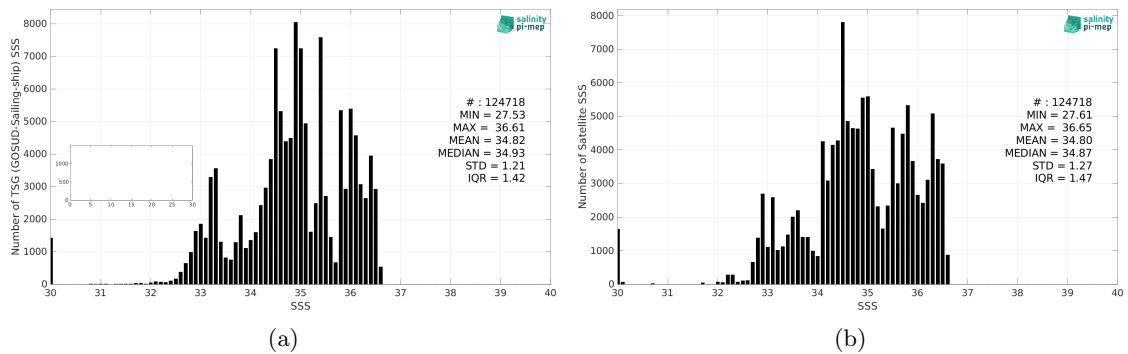
Figure 2: Histograms of SSS from TSG (GOSUD-Sailing-ship) (a) and SMOS SSS L3 v332 - 9 Days (CATDS-CPDC) (b) considering all match-up pairs per bins of 0.1 over the Tropical Pacific Ocean Pi-MEP region and for the full satellite product period.
