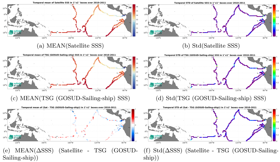
Figure 6: Temporal mean (left) and Std (right) of SSS from SMOS SSS L3 v332 - 9 Days (CATDS-CPDC) (top), TSG (GOSUD-Sailing-ship) (middle), and of \Delta SSS (Satellite - TSG (GOSUD-Sailing-ship)). Only match-up pairs are used to generate these maps.
