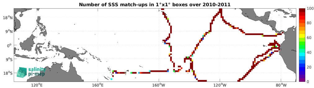
Figure 4: Number of SSS match-ups between TSG (GOSUD-Sailing-ship) SSS and the SMOS SSS L3 v332 - 9 Days (CATDS-CPDC) SSS product for the Tropical Pacific Ocean Pi-MEP region over 1^\circ \times 1^\circ boxes and for the full satellite product period.
