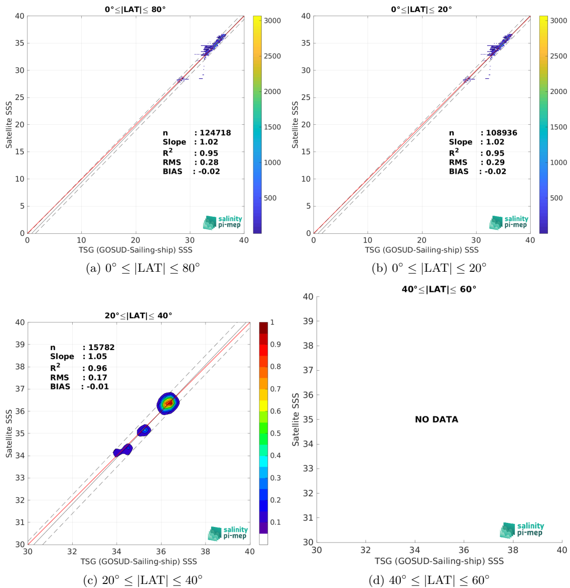
Figure 9: Contour maps of the concentration of SMOS SSS L3 v332 - 9 Days (CATDS-CPDC) SSS (y-axis) versus TSG (GOSUD-Sailing-ship) SSS (x-axis) at match-up pairs for different latitude bands. For each plot, the red line shows x=y . The black thin and dashed lines indicate a linear fit through the data cloud and the \pm 95\% confidence levels, respectively. The number match-up pairs n , the slope and R^2 coefficient of the linear fit, the root mean square (RMS) and the mean bias between satellite and in situ data are indicated for each latitude band in each plots.
