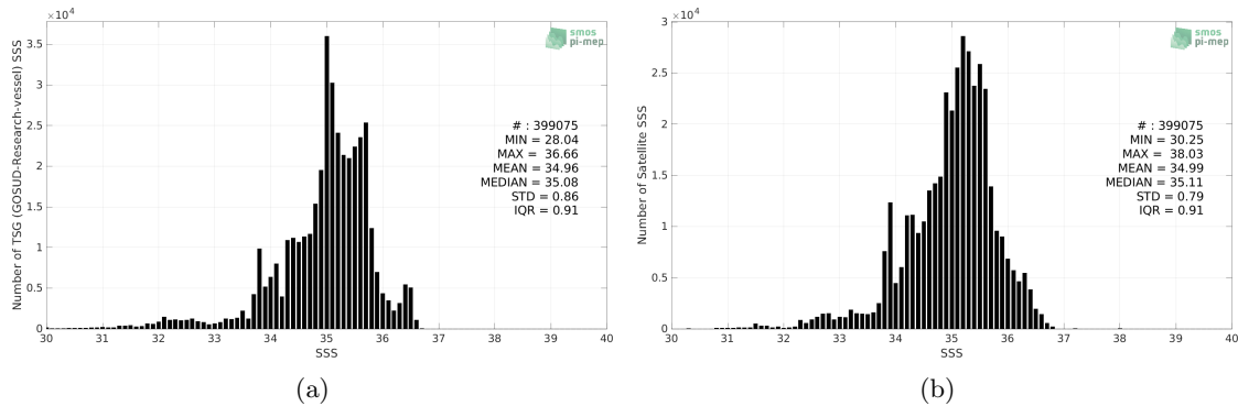
Figure 2: Histograms of SSS from TSG (GOSUD-Research-vessel) (a) and SMOS SSS L3 v332 - 9 Days (CATDS-CPDC) (b) considering all match-up pairs per bins of 0.1 over the Tropical Pacific Ocean Pi-MEP region and for the full satellite product period.
