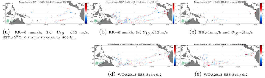
Figure 12: Temporal mean gridded over spatial boxes of size 1^{\circ}\times 1^{\circ} of \Delta SSS (SMOS SSS L3 v332 - 9 Days (CATDS-CPDC) - TSG (GOSUD-Research-vessel)) for 5 different subdatasets corresponding to:RR=0 mm/h, 3 < U_{10} < 12 m/s, SST >5^{\circ}\text{C} , distance to coast > 800 km (a), RR=0 mm/h, 3 < U_{10} < 12 m/s (b), RR >1 mm/h and U_{10} < 4 m/s (c), WOA2013 SSS Std <0.2 (d), WOA2013 SSS Std >0.2 (e).
