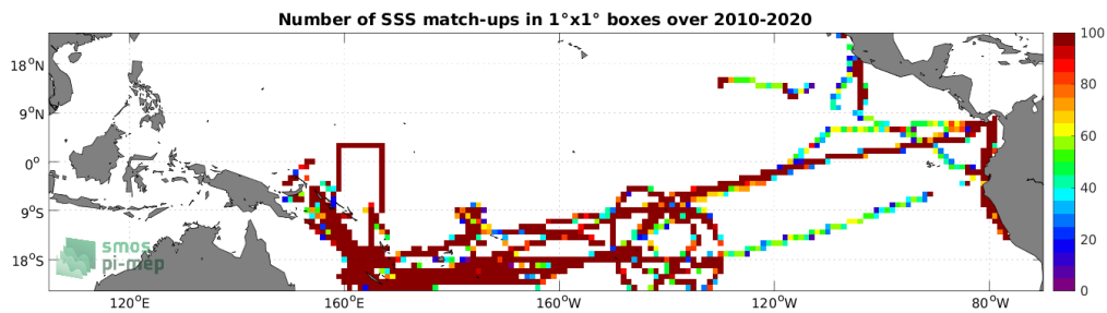
Figure 4: Number of SSS match-ups between TSG (GOSUD-Research-vessel) SSS and the SMOS SSS L3 v332 - 9 Days (CATDS-CPDC) SSS product for the Tropical Pacific Ocean Pi-MEP region over 1^\circ \times 1^\circ boxes and for the full satellite product period.
