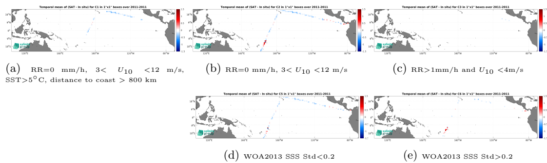
Figure 14: Temporal mean gridded over spatial boxes of size 1^\circ \times 1^\circ of \Delta SSS (SMOS SSS L3 v332 - 9 Days (CATDS-CPDC) - TSG (CSIC-UTM)) for 5 different subdatasets corresponding to: RR=0 mm/h, 3 < U_{10} < 12 m/s, SST > 5^\circ\text{C} , distance to coast > 800 km (a), RR=0 mm/h, 3 < U_{10} < 12 m/s (b), RR > 1 mm/h and U_{10} < 4 m/s (c), WOA2013 SSS Std < 0.2 (d), WOA2013 SSS Std > 0.2 (e).
