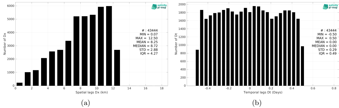
Figure 6: Histograms of the spatial (a) and temporal (b) lags between the location/time of the TSG (CSIC-UTM) measurement and the date of the corresponding SMOS SSS L3 v332 - 9 Days (CATDS-CPDC) SSS pixel.
