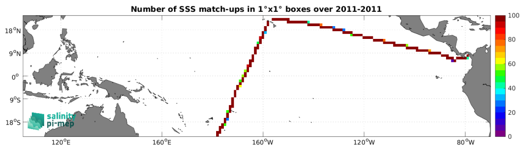
Figure 5: Number of SSS match-ups between TSG (CSIC-UTM) SSS and the SMOS SSS L3 v332 - 9 Days (CATDS-CPDC) SSS product for the Tropical Pacific Ocean Pi-MEP region over 1^\circ \times 1^\circ boxes and for the full satellite product period.
