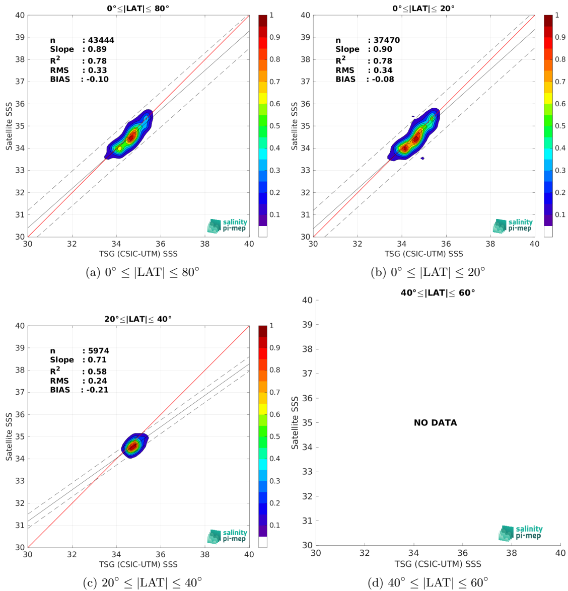
Figure 10: Contour maps of the concentration of SMOS SSS L3 v332 - 9 Days (CATDS-CPDC) SSS (y-axis) versus TSG (CSIC-UTM) SSS (x-axis) at match-up pairs for different latitude bands. For each plot, the red line shows x=y . The black thin and dashed lines indicate a linear fit through the data cloud and the \pm 95\% confidence levels, respectively. The number match-up pairs n , the slope and R^2 coefficient of the linear fit, the root mean square (RMS) and the mean bias between satellite and in situ data are indicated for each latitude band in each plots.
