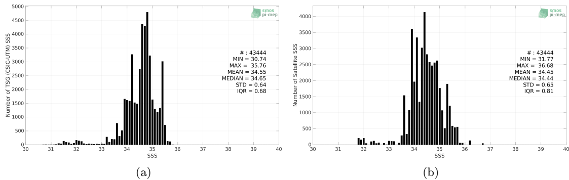
Figure 2: Histograms of SSS from TSG (CSIC-UTM) (a) and SMOS SSS L3 v332 - 9 Days (CATDS-CPDC) (b) considering all match-up pairs per bins of 0.1 over the Tropical Pacific Ocean Pi-MEP region and for the full satellite product period.
