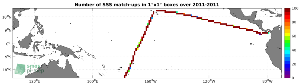
Figure 4: Number of SSS match-ups between TSG (CSIC-UTM) SSS and the SMOS SSS L3 v332 - 9 Days (CATDS-CPDC) SSS product for the Tropical Pacific Ocean Pi-MEP region over 1^\circ \times 1^\circ boxes and for the full satellite product period.
