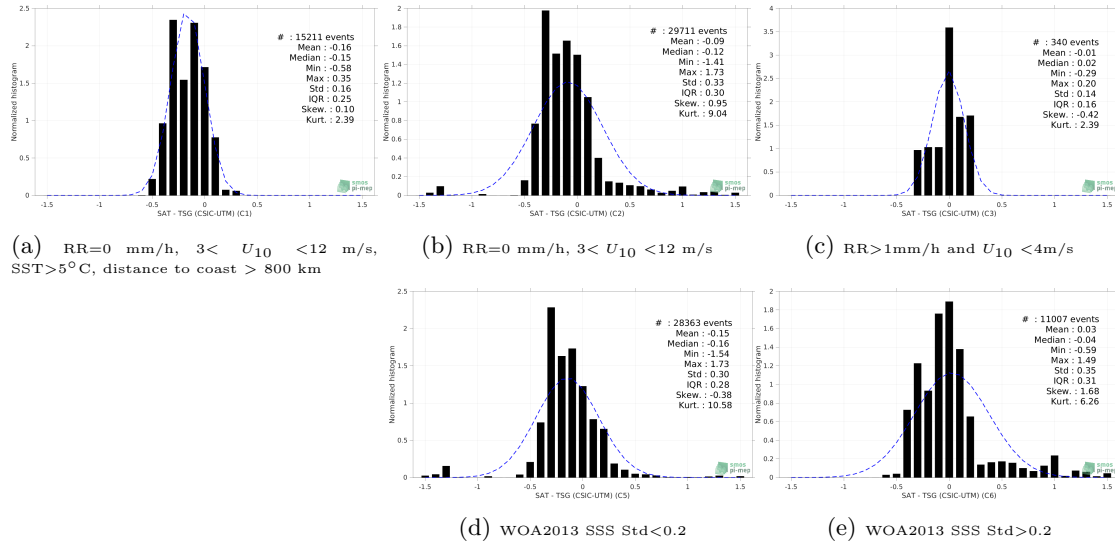
Figure 13: Normalized histogram of \Delta SSS (SMOS SSS L3 v332 - 9 Days (CATDS-CPDC) - TSG (CSIC-UTM)) for 5 different subdatasets corresponding to: RR=0 mm/h, 3 < U_{10} < 12 m/s, SST > 5°C, distance to coast > 800 km (a), RR=0 mm/h, 3 < U_{10} < 12 m/s (b), RR > 1mm/h and U_{10} < 4 m/s (c), WOA2013 SSS Std < 0.2 (d), WOA2013 SSS Std > 0.2 (e).
