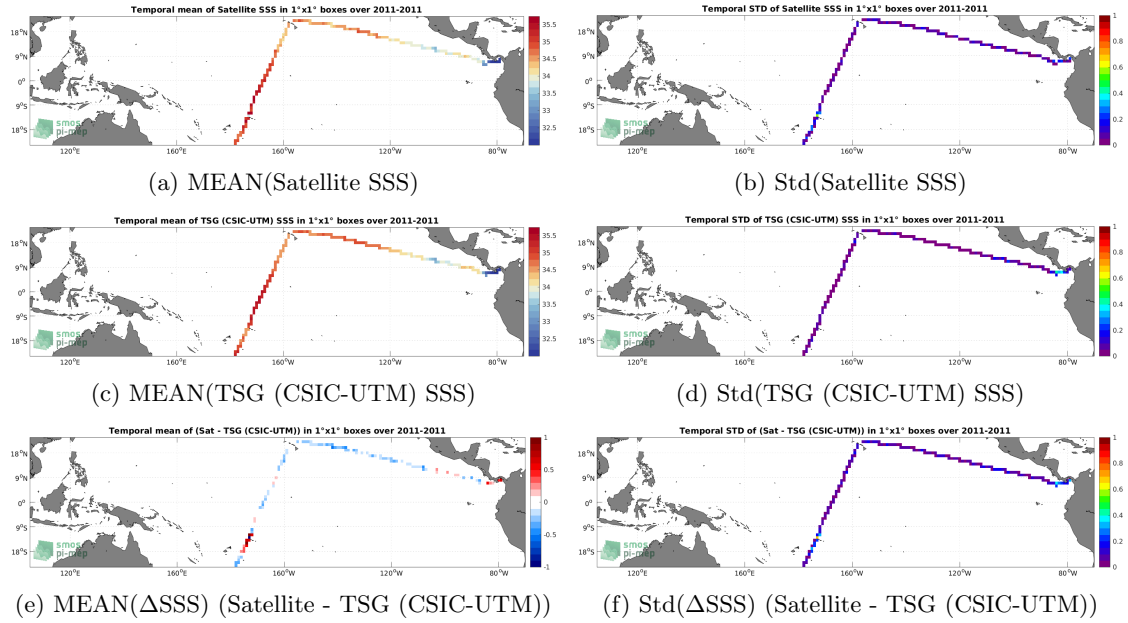
Figure 6: Temporal mean (left) and Std (right) of SSS from SMOS SSS L3 v332 - 9 Days (CATDS-CPDC) (top), TSG (CSIC-UTM) (middle), and of \Delta SSS (Satellite - TSG (CSIC-UTM)). Only match-up pairs are used to generate these maps.
