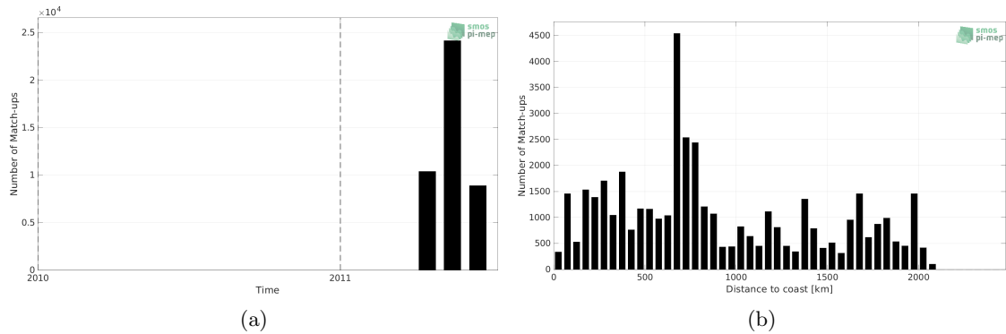
Figure 1: Number of match-ups between TSG (CSIC-UTM) and SMOS SSS L3 v332 - 9 Days (CATDS-CPDC) SSS as a function of time (a) and as function of the distance to coast (b) over the Tropical Pacific Ocean Pi-MEP region and for the full satellite product period.
