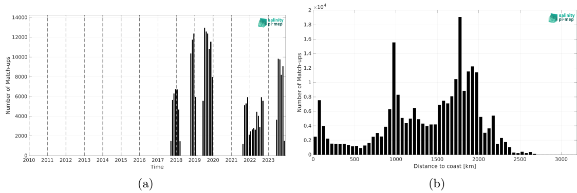
Figure 2: Number of match-ups between Saildrone and SMOS SSS L3 v332 - 9 Days (CATDS-CPDC) SSS as a function of time (a) and as function of the distance to coast (b) over the Tropical Pacific Ocean Pi-MEP region and for the full satellite product period.
