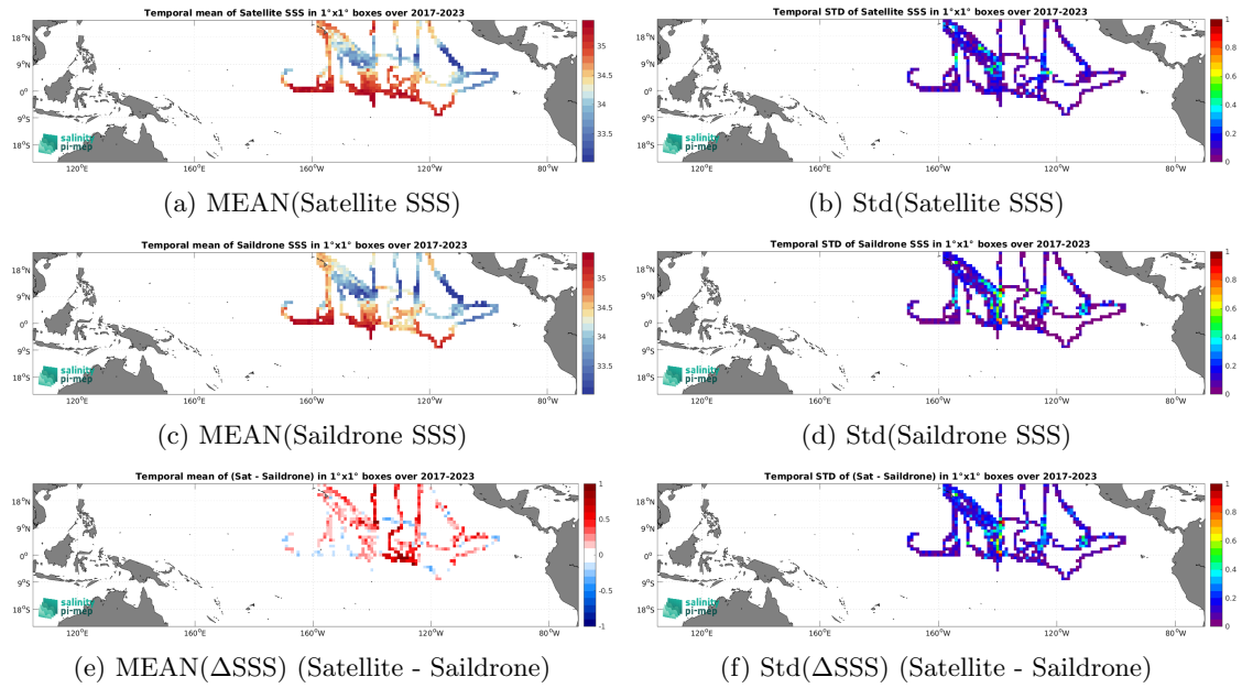
Figure 7: Temporal mean (left) and Std (right) of SSS from SMOS SSS L3 v332 - 9 Days (CATDS-CPDC) (top), Saildrone (middle), and of \Delta SSS (Satellite - Saildrone). Only match-up pairs are used to generate these maps.
