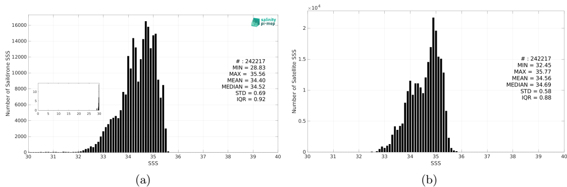
Figure 3: Histograms of SSS from Saildrone (a) and SMOS SSS L3 v332 - 9 Days (CATDS-CPDC) (b) considering all match-up pairs per bins of 0.1 over the Tropical Pacific Ocean Pi-MEP region and for the full satellite product period.
