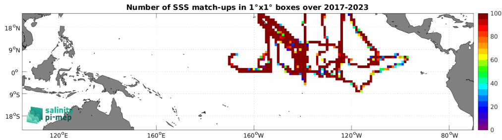
Figure 5: Number of SSS match-ups between Saildrone SSS and the SMOS SSS L3 v332 - 9 Days (CATDS-CPDC) SSS product for the Tropical Pacific Ocean Pi-MEP region over 1^\circ \times 1^\circ boxes and for the full satellite product period.
