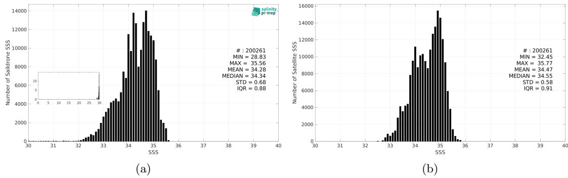
Figure 3: Histograms of SSS from Saildrone (a) and SMOS SSS L3 v332 - 9 Days (CATDS-CPDC) (b) considering all match-up pairs per bins of 0.1 over the Tropical Pacific Ocean Pi-MEP region and for the full satellite product period.
