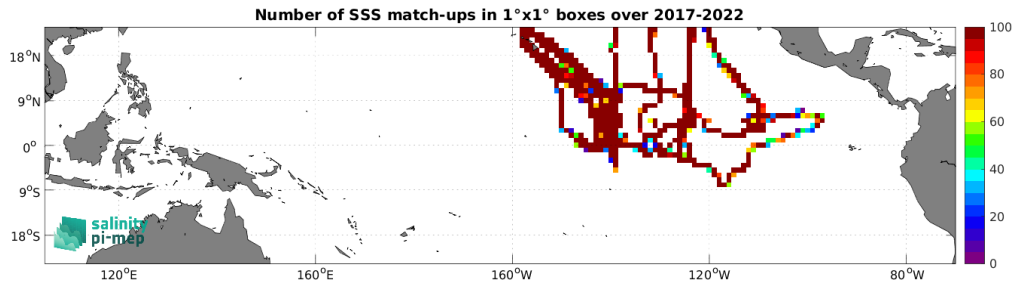
Figure 5: Number of SSS match-ups between Saildrone SSS and the SMOS SSS L3 v332 - 9 Days (CATDS-CPDC) SSS product for the Tropical Pacific Ocean Pi-MEP region over 1^\circ \times 1^\circ boxes and for the full satellite product period.
