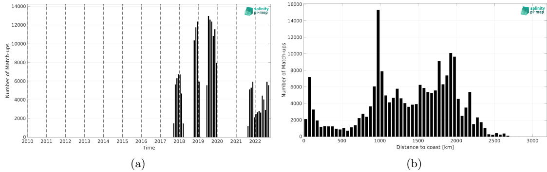
Figure 2: Number of match-ups between Saildrone and SMOS SSS L3 v332 - 9 Days (CATDS-CPDC) SSS as a function of time (a) and as function of the distance to coast (b) over the Tropical Pacific Ocean Pi-MEP region and for the full satellite product period.
