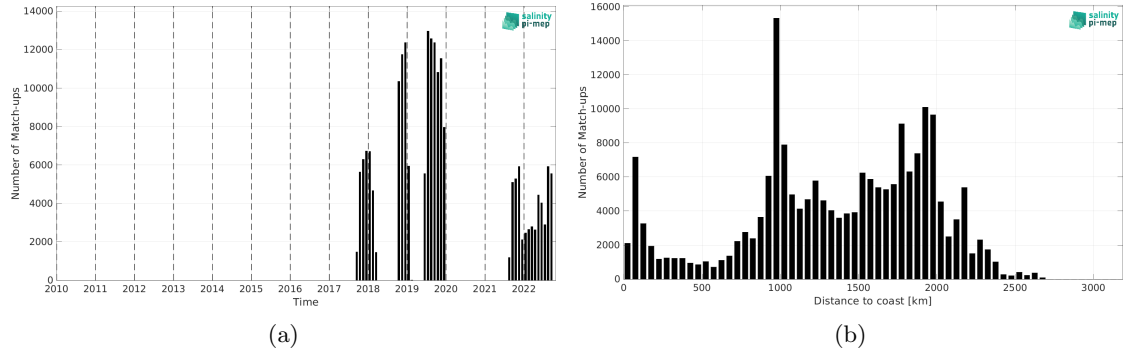
Figure 1: Number of match-ups between Saildrone and SMOS SSS L3 v332 - 9 Days (CATDS-CPDC) SSS as a function of time (a) and as function of the distance to coast (b) over the Tropical Pacific Ocean Pi-MEP region and for the full satellite product period.
