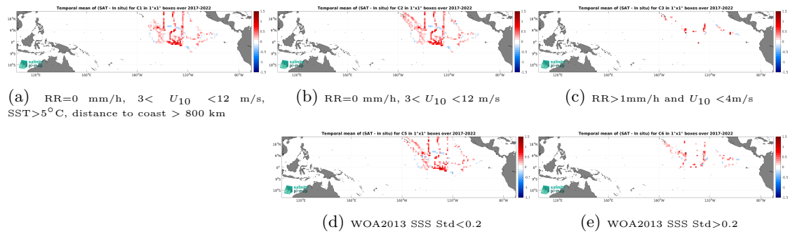
Figure 12: Temporal mean gridded over spatial boxes of size 1^\circ \times 1^\circ of \Delta SSS (SMOS SSS L3 v332 - 9 Days (CATDS-CPDC) - Saildrone) for 5 different subdatasets corresponding to:RR=0 mm/h, 3 < U_{10} < 12 m/s, SST > 5^\circ\text{C} , distance to coast > 800 km (a), RR=0 mm/h, 3 < U_{10} < 12 m/s (b), RR > 1 mm/h and U_{10} < 4 m/s (c), WOA2013 SSS Std < 0.2 (d), WOA2013 SSS Std > 0.2 (e).
