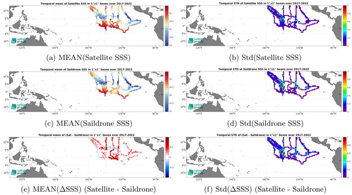
Figure 6: Temporal mean (left) and Std (right) of SSS from SMOS SSS L3 v332 - 9 Days (CATDS-CPDC) (top), Saildrone (middle), and of \Delta SSS (Satellite - Saildrone). Only match-up pairs are used to generate these maps.
