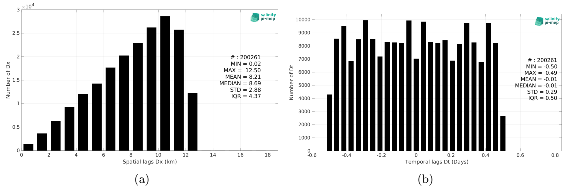
Figure 5: Histograms of the spatial (a) and temporal (b) lags between the location/time of the Saildrone measurement and the date of the corresponding SMOS SSS L3 v332 - 9 Days (CATDS-CPDC) SSS pixel.
