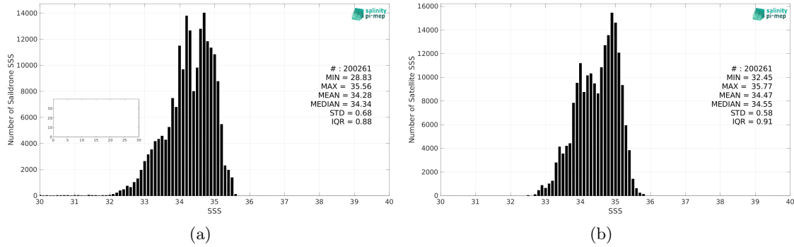
Figure 2: Histograms of SSS from Saildrone (a) and SMOS SSS L3 v332 - 9 Days (CATDS-CPDC) (b) considering all match-up pairs per bins of 0.1 over the Tropical Pacific Ocean Pi-MEP region and for the full satellite product period.
