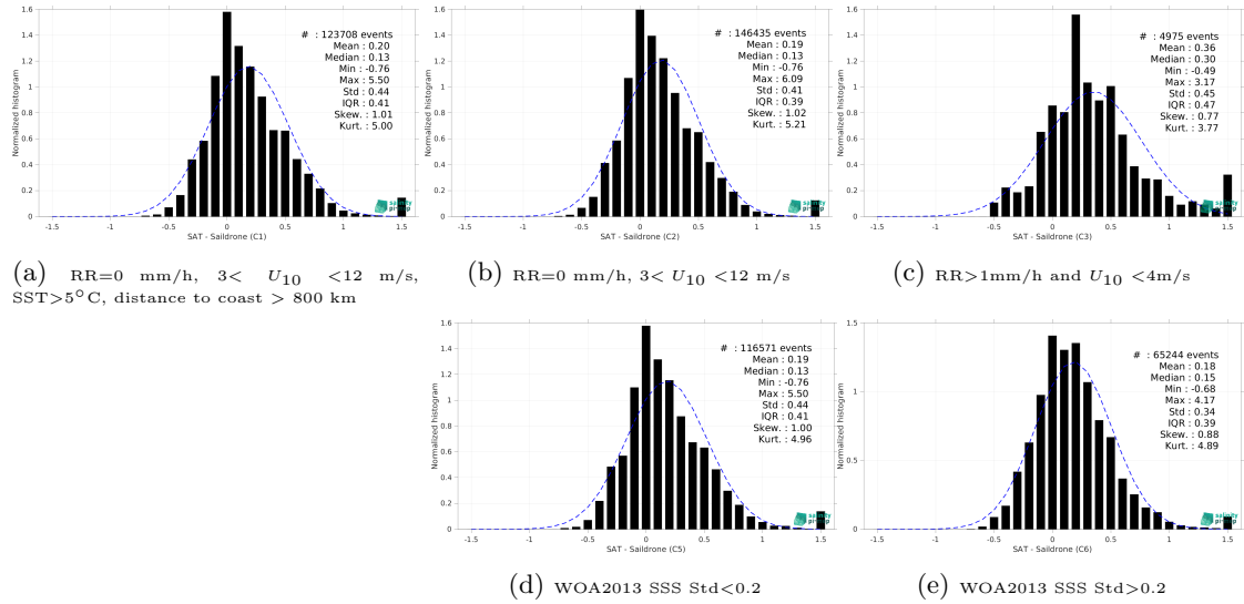
Figure 13: Normalized histogram of \Delta SSS (SMOS SSS L3 v332 - 9 Days (CATDS-CPDC) - Saildrone) for 5 different subdatasets corresponding to: RR=0 mm/h, 3 < U_{10} < 12 m/s, SST>5°C, distance to coast > 800 km (a), RR=0 mm/h, 3 < U_{10} < 12 m/s (b), RR>1mm/h and U_{10} < 4 m/s (c), WOA2013 SSS Std<0.2 (d), WOA2013 SSS Std>0.2 (e).
