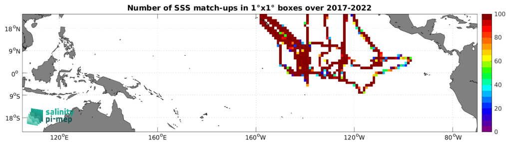
Figure 4: Number of SSS match-ups between Saildrone SSS and the SMOS SSS L3 v332 - 9 Days (CATDS-CPDC) SSS product for the Tropical Pacific Ocean Pi-MEP region over 1^\circ \times 1^\circ boxes and for the full satellite product period.
