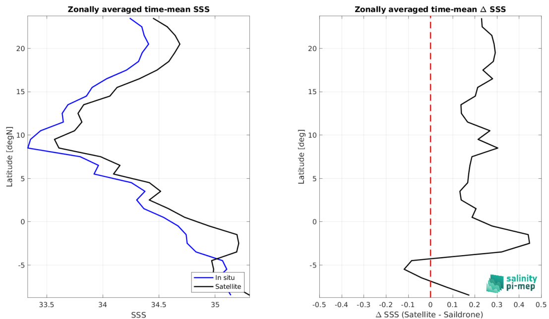
Figure 8: Left panel: Zonal mean SSS from SMOS SSS L3 v332 - 9 Days (CATDS-CPDC) satellite product (black) and from Saildrone (blue). Right panel: Zonal mean of \Delta SSS (Satellite - Saildrone) for all the collected Pi-MEP match-up pairs estimated over the full satellite product period.
