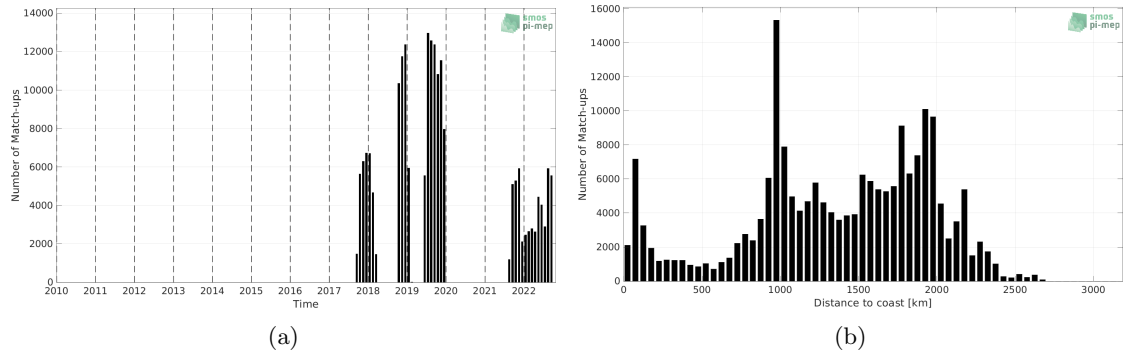
Figure 1: Number of match-ups between Saildrone and SMOS SSS L3 v332 - 9 Days (CATDS-CPDC) SSS as a function of time (a) and as function of the distance to the coast (b) over the Tropical Pacific Ocean Pi-MEP region and for the full satellite product period.
