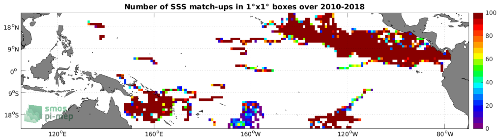
Figure 3: Number of SSS match-ups between Surface drifters SSS and the SMOS SSS L3 v332 - 9 Days (CATDS-CPDC) SSS product for the Tropical Pacific Ocean Pi-MEP region over 1^\circ \times 1^\circ boxes and for the full satellite product period.
