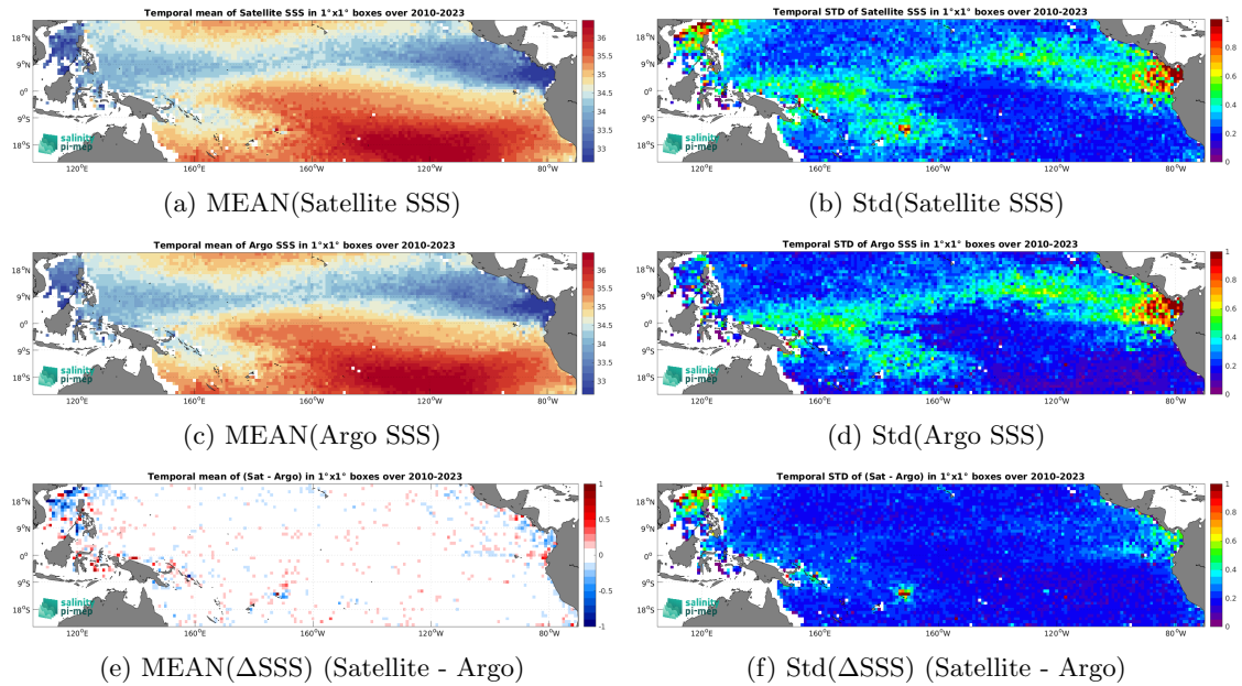
Figure 6: Temporal mean (left) and Std (right) of SSS from SMOS SSS L3 v332 - 9 Days (CATDS-CPDC) (top), Argo (middle), and of \Delta SSS (Satellite - Argo). Only match-up pairs are used to generate these maps.
