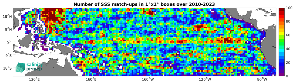
Figure 4: Number of SSS match-ups between Argo SSS and the SMOS SSS L3 v332 - 9 Days (CATDS-CPDC) SSS product for the Tropical Pacific Ocean Pi-MEP region over 1^\circ \times 1^\circ boxes and for the full satellite product period.
