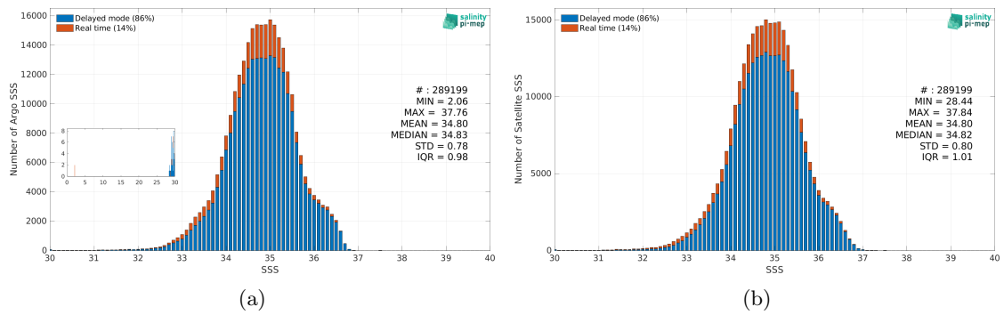
Figure 2: Histograms of SSS from Argo (a) and SMOS SSS L3 v332 - 9 Days (CATDS-CPDC) (b) considering all match-up pairs per bins of 0.1 over the Tropical Pacific Ocean Pi-MEP region and for the full satellite product period.
