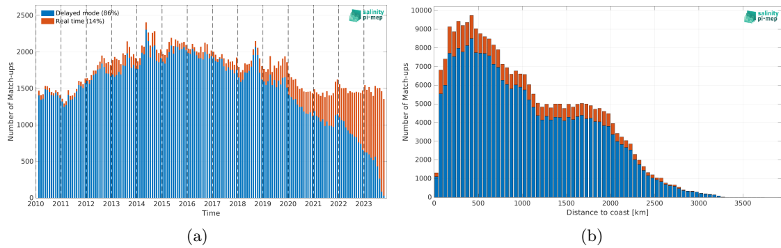
Figure 1: Number of match-ups between Argo and SMOS SSS L3 v332 - 9 Days (CATDS-CPDC) SSS as a function of time (a) and as function of the distance to coast (b) over the Tropical Pacific Ocean Pi-MEP region and for the full satellite product period.
