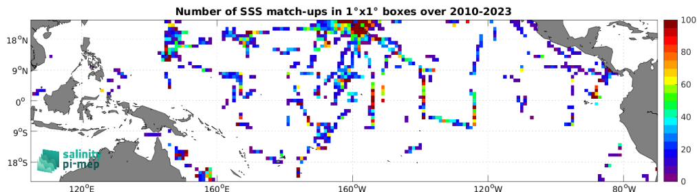
Figure 4: Number of SSS match-ups between TSG (SAMOS) SSS and the SMOS SSS L2Q v331 - 0.25 Deg (CATDS-CPDC) SSS product for the Tropical Pacific Ocean Pi-MEP region over 1^\circ \times 1^\circ boxes and for the full satellite product period.
