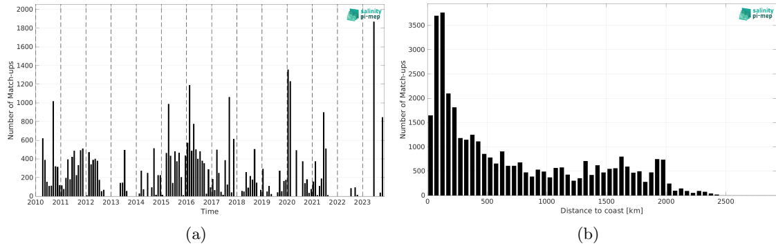
Figure 1: Number of match-ups between TSG (SAMOS) and SMOS SSS L2Q v331 - 0.25 Deg (CATDS-CPDC) SSS as a function of time (a) and as function of the distance to coast (b) over the Tropical Pacific Ocean Pi-MEP region and for the full satellite product period.
