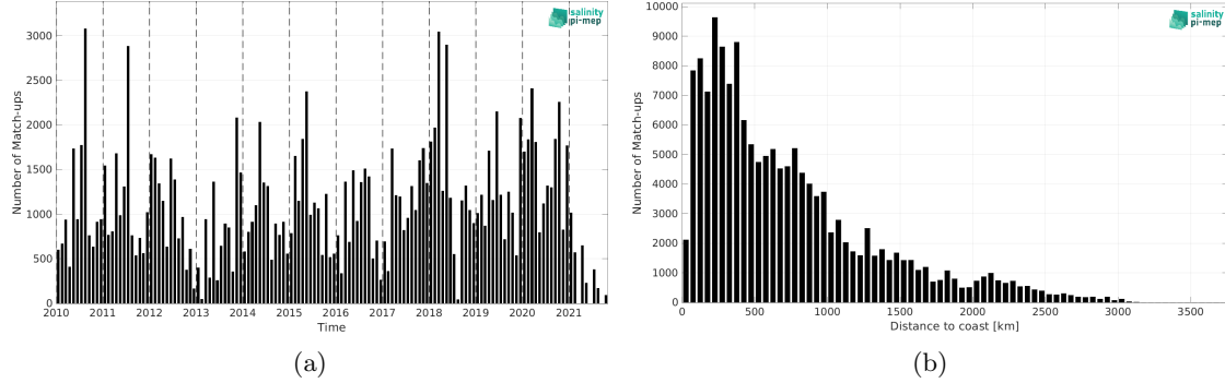
Figure 1: Number of match-ups between TSG (LEGOS-DM) and SMOS SSS L2Q v331 - 0.25 Deg (CATDS-CPDC) SSS as a function of time (a) and as function of the distance to coast (b) over the Tropical Pacific Ocean Pi-MEP region and for the full satellite product period.
