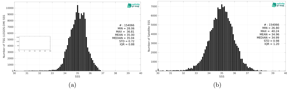
Figure 2: Histograms of SSS from TSG (LEGOS-DM) (a) and SMOS SSS L2Q v331 - 0.25 Deg (CATDS-CPDC) (b) considering all match-up pairs per bins of 0.1 over the Tropical Pacific Ocean Pi-MEP region and for the full satellite product period.
