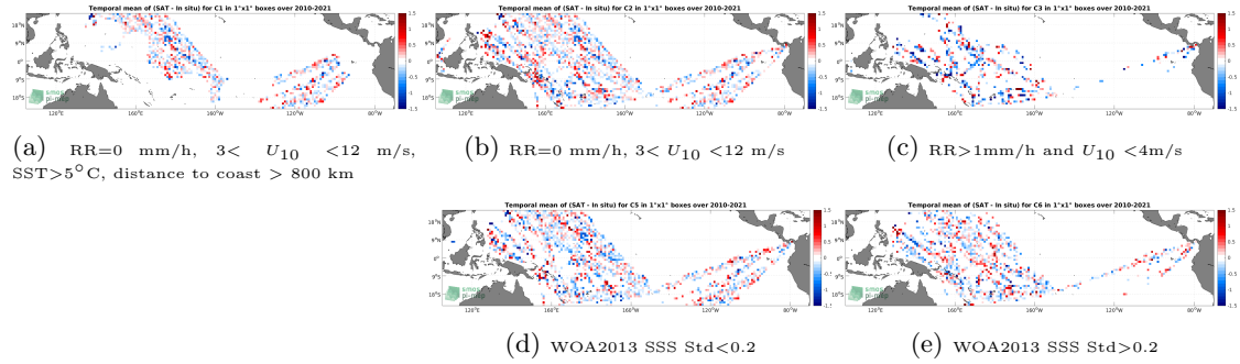
Figure 12: Temporal mean gridded over spatial boxes of size 1^{\circ}\times 1^{\circ} of \Delta\text{SSS} (SMOS SSS L2Q v331 - 0.25 Deg (CATDS-CPDC) - TSG (LEGOS-DM)) for 5 different subdatasets corresponding to:RR=0 mm/h, 3 < U_{10} < 12 m/s, SST > 5^{\circ}\text{C} , distance to coast > 800 km (a), RR=0 mm/h, 3 < U_{10} < 12 m/s (b), RR > 1 mm/h and U_{10} < 4 m/s (c), WOA2013 SSS Std < 0.2 (d), WOA2013 SSS Std > 0.2 (e).
