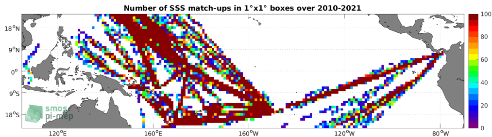
Figure 4: Number of SSS match-ups between TSG (LEGOS-DM) SSS and the SMOS SSS L2Q v331 - 0.25 Deg (CATDS-CPDC) SSS product for the Tropical Pacific Ocean Pi-MEP region over 1^\circ \times 1^\circ boxes and for the full satellite product period.
