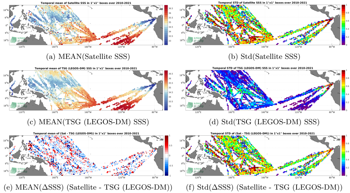
Figure 6: Temporal mean (left) and Std (right) of SSS from SMOS SSS L2Q v331 - 0.25 Deg (CATDS-CPDC) (top), TSG (LEGOS-DM) (middle), and of \Delta SSS (Satellite - TSG (LEGOS-DM)). Only match-up pairs are used to generate these maps.
