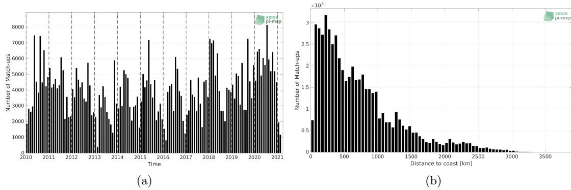
Figure 1: Number of match-ups between TSG (LEGOS-DM) and SMOS SSS L2Q v331 - 0.25 Deg (CATDS-CPDC) SSS as a function of time (a) and as function of the distance to coast (b) over the Tropical Pacific Ocean Pi-MEP region and for the full satellite product period.
