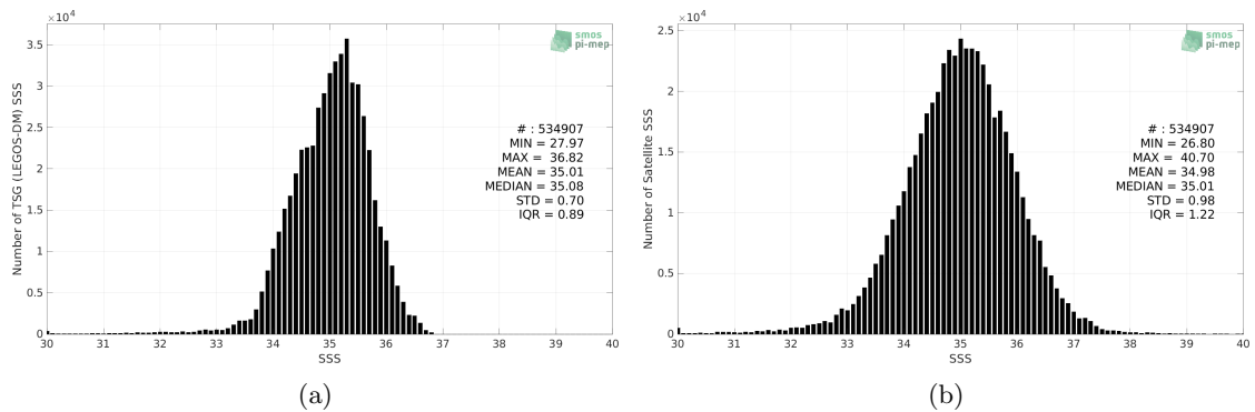
Figure 2: Histograms of SSS from TSG (LEGOS-DM) (a) and SMOS SSS L2Q v331 - 0.25 Deg (CATDS-CPDC) (b) considering all match-up pairs per bins of 0.1 over the Tropical Pacific Ocean Pi-MEP region and for the full satellite product period.
