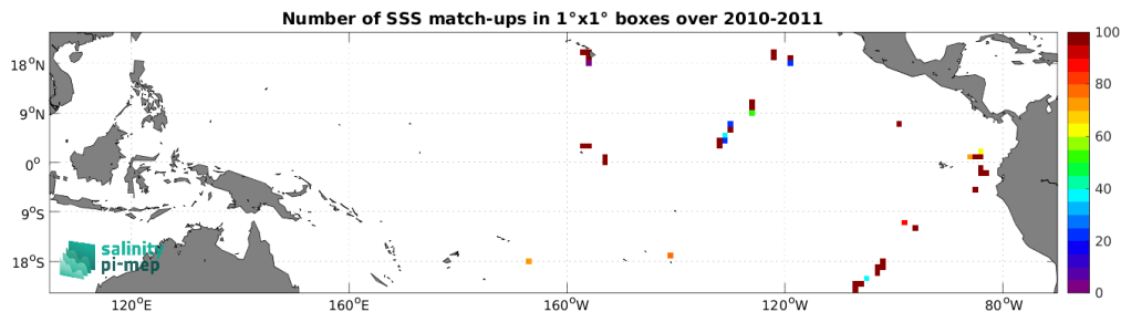
Figure 4: Number of SSS match-ups between TSG (GOSUD-Sailing-ship) SSS and the SMOS SSS L2Q v331 - 0.25 Deg (CATDS-CPDC) SSS product for the Tropical Pacific Ocean Pi-MEP region over 1^\circ \times 1^\circ boxes and for the full satellite product period.
