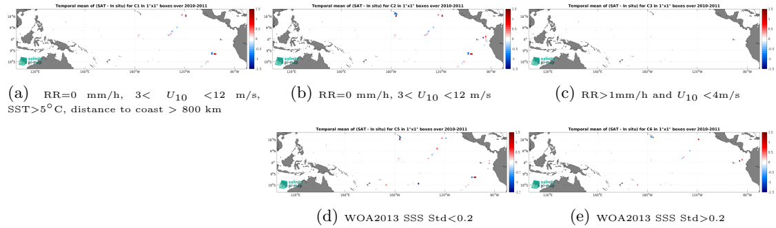
Figure 12: Temporal mean gridded over spatial boxes of size 1^{\circ}\times 1^{\circ} of \Delta SSS (SMOS SSS L2Q v331 - 0.25 Deg (CATDS-CPDC) - TSG (GOSUD-Sailing-ship)) for 5 different subdatasets corresponding to:RR=0 mm/h, 3 < U_{10} < 12 m/s, SST >5^{\circ}\text{C} , distance to coast > 800 km (a), RR=0 mm/h, 3 < U_{10} < 12 m/s (b), RR >1 mm/h and U_{10} < 4 m/s (c), WOA2013 SSS Std <0.2 (d), WOA2013 SSS Std >0.2 (e).
