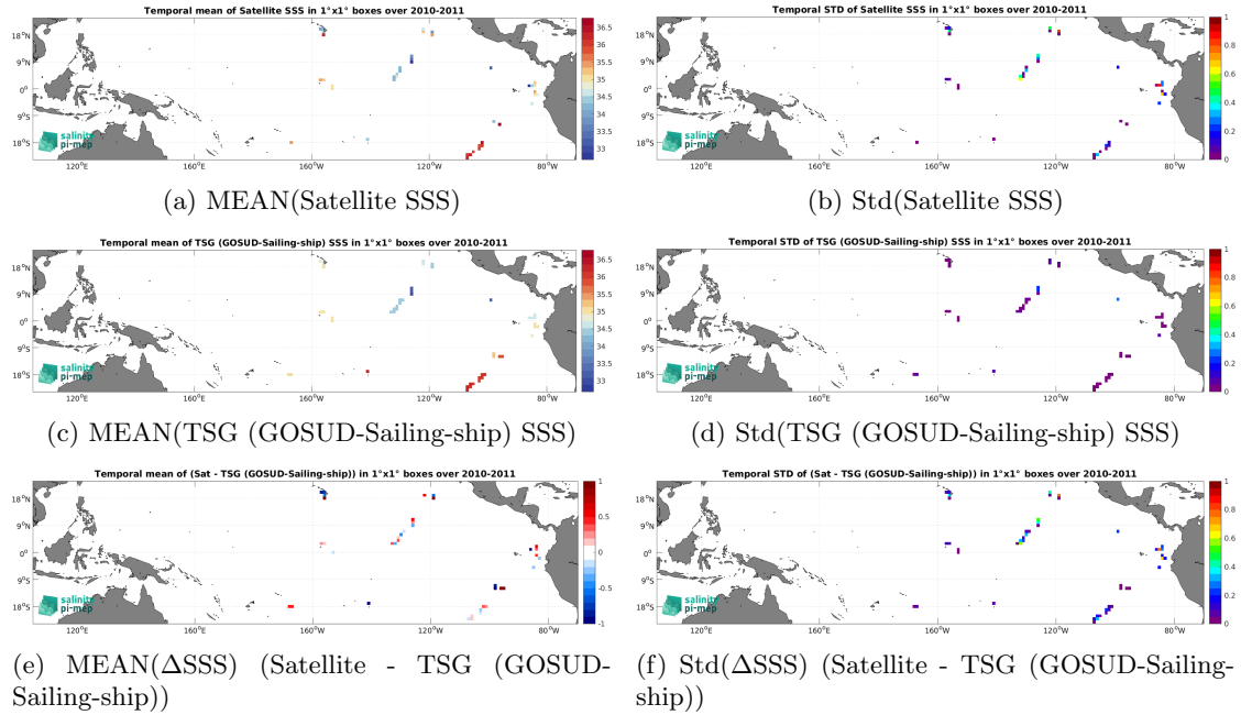
Figure 6: Temporal mean (left) and Std (right) of SSS from SMOS SSS L2Q v331 - 0.25 Deg (CATDS-CPDC) (top), TSG (GOSUD-Sailing-ship) (middle), and of \Delta SSS (Satellite - TSG (GOSUD-Sailing-ship)). Only match-up pairs are used to generate these maps.
