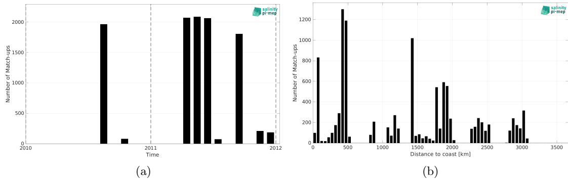
Figure 1: Number of match-ups between TSG (GOSUD-Sailing-ship) and SMOS SSS L2Q v331 - 0.25 Deg (CATDS-CPDC) SSS as a function of time (a) and as function of the distance to coast (b) over the Tropical Pacific Ocean Pi-MEP region and for the full satellite product period.
