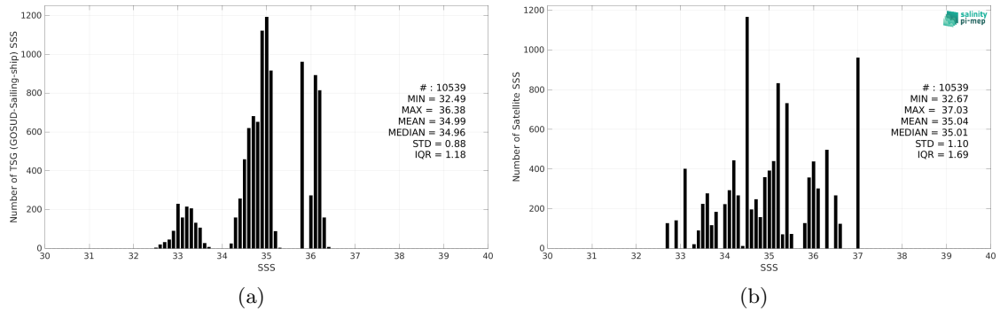
Figure 2: Histograms of SSS from TSG (GOSUD-Sailing-ship) (a) and SMOS SSS L2Q v331 - 0.25 Deg (CATDS-CPDC) (b) considering all match-up pairs per bins of 0.1 over the Tropical Pacific Ocean Pi-MEP region and for the full satellite product period.
