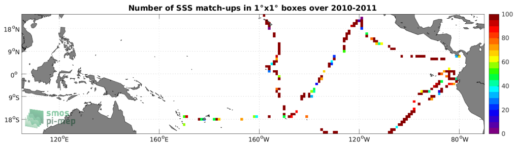
Figure 4: Number of SSS match-ups between TSG (GOSUD-Sailing-ship) SSS and the SMOS SSS L2Q v331 - 0.25 Deg (CATDS-CPDC) SSS product for the Tropical Pacific Ocean Pi-MEP region over 1^\circ \times 1^\circ boxes and for the full satellite product period.
