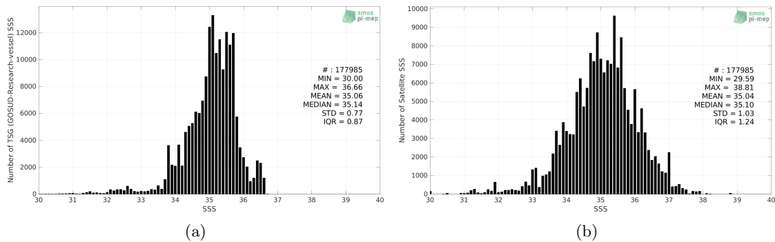
Figure 2: Histograms of SSS from TSG (GOSUD-Research-vessel) (a) and SMOS SSS L2Q v331 - 0.25 Deg (CATDS-CPDC) (b) considering all match-up pairs per bins of 0.1 over the Tropical Pacific Ocean Pi-MEP region and for the full satellite product period.
