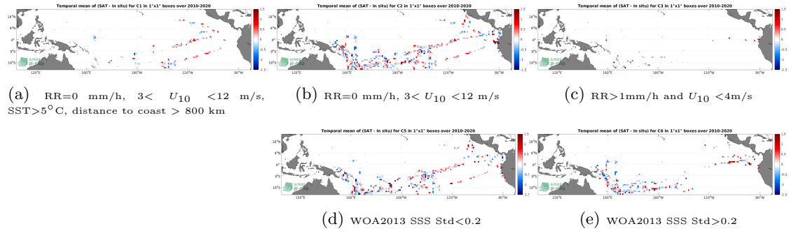
Figure 12: Temporal mean gridded over spatial boxes of size 1^{\circ}\times 1^{\circ} of \Delta SSS (SMOS SSS L2Q v331 - 0.25 Deg (CATDS-CPDC) - TSG (GOSUD-Research-vessel)) for 5 different subdatasets corresponding to:RR=0 mm/h, 3 < U_{10} < 12 m/s, SST >5^{\circ}\text{C} , distance to coast > 800 km (a), RR=0 mm/h, 3 < U_{10} < 12 m/s (b), RR >1 mm/h and U_{10} < 4 m/s (c), WOA2013 SSS Std <0.2 (d), WOA2013 SSS Std >0.2 (e).
