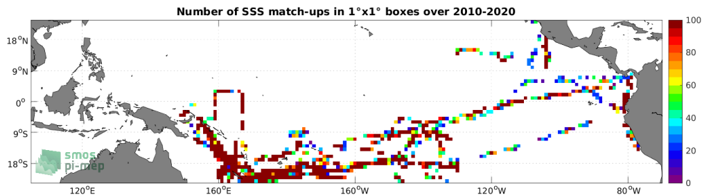
Figure 4: Number of SSS match-ups between TSG (GOSUD-Research-vessel) SSS and the SMOS SSS L2Q v331 - 0.25 Deg (CATDS-CPDC) SSS product for the Tropical Pacific Ocean Pi-MEP region over 1^\circ \times 1^\circ boxes and for the full satellite product period.
