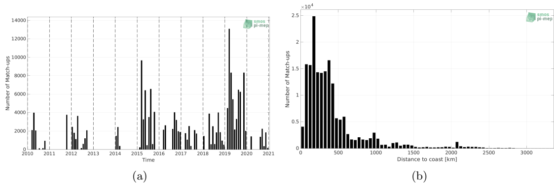
Figure 1: Number of match-ups between TSG (GOSUD-Research-vessel) and SMOS SSS L2Q v331 - 0.25 Deg (CATDS-CPDC) SSS as a function of time (a) and as function of the distance to coast (b) over the Tropical Pacific Ocean Pi-MEP region and for the full satellite product period.
