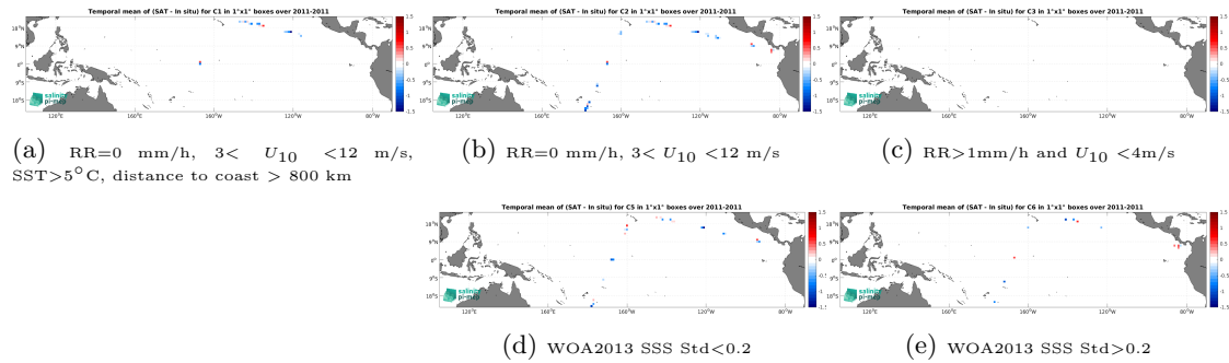
Figure 12: Temporal mean gridded over spatial boxes of size 1^{\circ}\times 1^{\circ} of \Delta\text{SSS} (SMOS SSS L2Q v331 - 0.25 Deg (CATDS-CPDC) - TSG (CSIC-UTM)) for 5 different subdatasets corresponding to:RR=0 mm/h, 3 < U_{10} < 12 m/s, SST > 5^{\circ}\text{C} , distance to coast > 800 km (a), RR=0 mm/h, 3 < U_{10} < 12 m/s (b), RR > 1 mm/h and U_{10} < 4 m/s (c), WOA2013 SSS Std < 0.2 (d), WOA2013 SSS Std > 0.2 (e).
