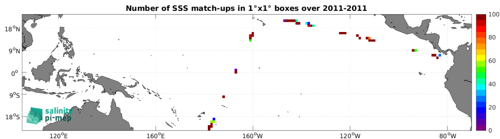
Figure 4: Number of SSS match-ups between TSG (CSIC-UTM) SSS and the SMOS SSS L2Q v331 - 0.25 Deg (CATDS-CPDC) SSS product for the Tropical Pacific Ocean Pi-MEP region over 1^\circ \times 1^\circ boxes and for the full satellite product period.
