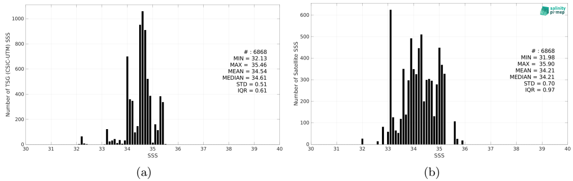
Figure 2: Histograms of SSS from TSG (CSIC-UTM) (a) and SMOS SSS L2Q v331 - 0.25 Deg (CATDS-CPDC) (b) considering all match-up pairs per bins of 0.1 over the Tropical Pacific Ocean Pi-MEP region and for the full satellite product period.
