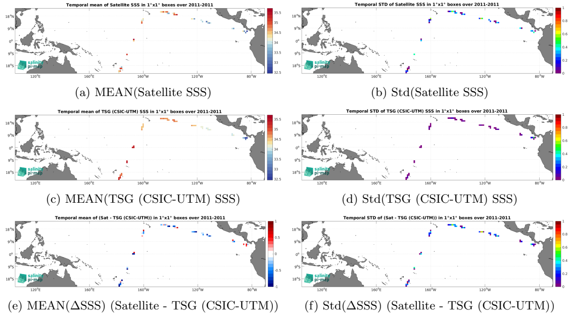
Figure 6: Temporal mean (left) and Std (right) of SSS from SMOS SSS L2Q v331 - 0.25 Deg (CATDS-CPDC) (top), TSG (CSIC-UTM) (middle), and of \Delta SSS (Satellite - TSG (CSIC-UTM)). Only match-up pairs are used to generate these maps.
