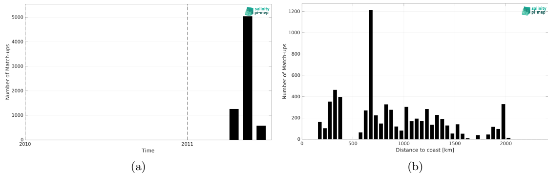
Figure 1: Number of match-ups between TSG (CSIC-UTM) and SMOS SSS L2Q v331 - 0.25 Deg (CATDS-CPDC) SSS as a function of time (a) and as function of the distance to coast (b) over the Tropical Pacific Ocean Pi-MEP region and for the full satellite product period.
