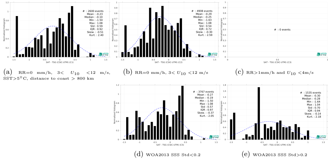
Figure 13: Normalized histogram of \Delta SSS (SMOS SSS L2Q v331 - 0.25 Deg (CATDS-CPDC) - TSG (CSIC-UTM)) for 5 different subdatasets corresponding to: RR=0 mm/h, 3 < U_{10} < 12 m/s, SST>5°C, distance to coast > 800 km (a), RR=0 mm/h, 3 < U_{10} < 12 m/s (b), RR>1mm/h and U_{10} < 4 m/s (c), WOA2013 SSS Std<0.2 (d), WOA2013 SSS Std>0.2 (e).
