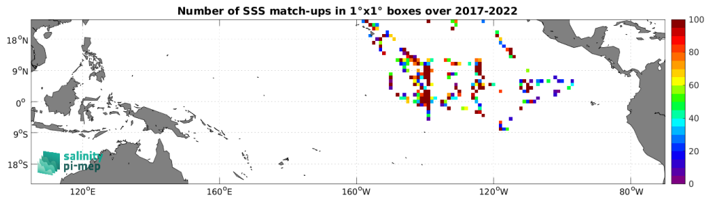
Figure 4: Number of SSS match-ups between Sairdrone SSS and the SMOS SSS L2Q v331 - 0.25 Deg (CATDS-CPDC) SSS product for the Tropical Pacific Ocean Pi-MEP region over 1^\circ \times 1^\circ boxes and for the full satellite product period.
