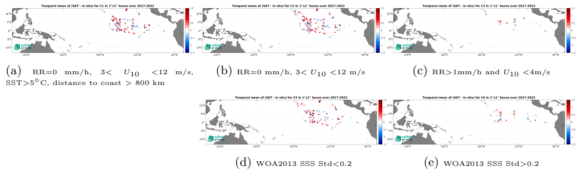
Figure 12: Temporal mean gridded over spatial boxes of size 1^\circ \times 1^\circ of \Delta SSS (SMOS SSS L2Q v331 - 0.25 Deg (CATDS-CPDC) - Saildrone) for 5 different subdatasets corresponding to:RR=0 mm/h, 3 < U_{10} < 12 m/s, SST > 5^\circ\text{C} , distance to coast > 800 km (a), RR=0 mm/h, 3 < U_{10} < 12 m/s (b), RR > 1 mm/h and U_{10} < 4 m/s (c), WOA2013 SSS Std < 0.2 (d), WOA2013 SSS Std > 0.2 (e).
