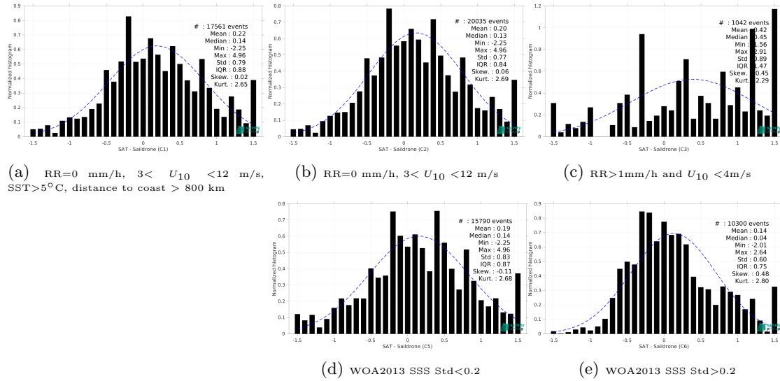
Figure 13: Normalized histogram of \Delta SSS (SMOS SSS L2Q v331 - 0.25 Deg (CATDS-CPDC) - Sairdronne) for 5 different subdatasets corresponding to: RR=0 mm/h, 3 < U_{10} < 12 m/s, SST > 5°C, distance to coast > 800 km (a), RR=0 mm/h, 3 < U_{10} < 12 m/s (b), RR > 1mm/h and U_{10} < 4 m/s (c), WOA2013 SSS Std < 0.2 (d), WOA2013 SSS Std > 0.2 (e).
