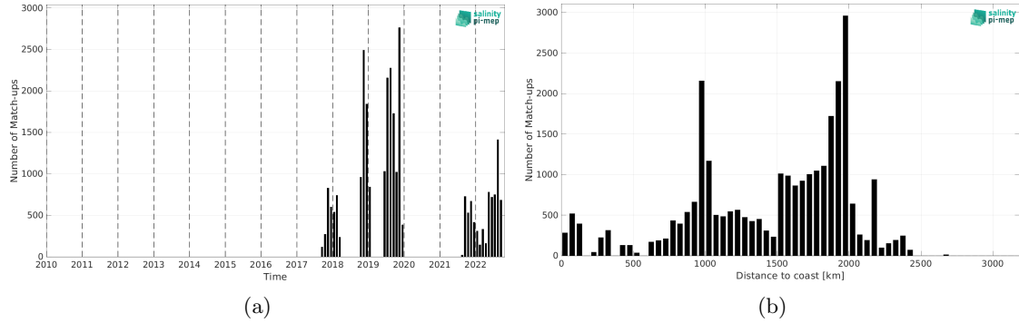
Figure 1: Number of match-ups between Saildrone and SMOS SSS L2Q v331 - 0.25 Deg (CATDS-CPDC) SSS as a function of time (a) and as function of the distance to coast (b) over the Tropical Pacific Ocean Pi-MEP region and for the full satellite product period.
