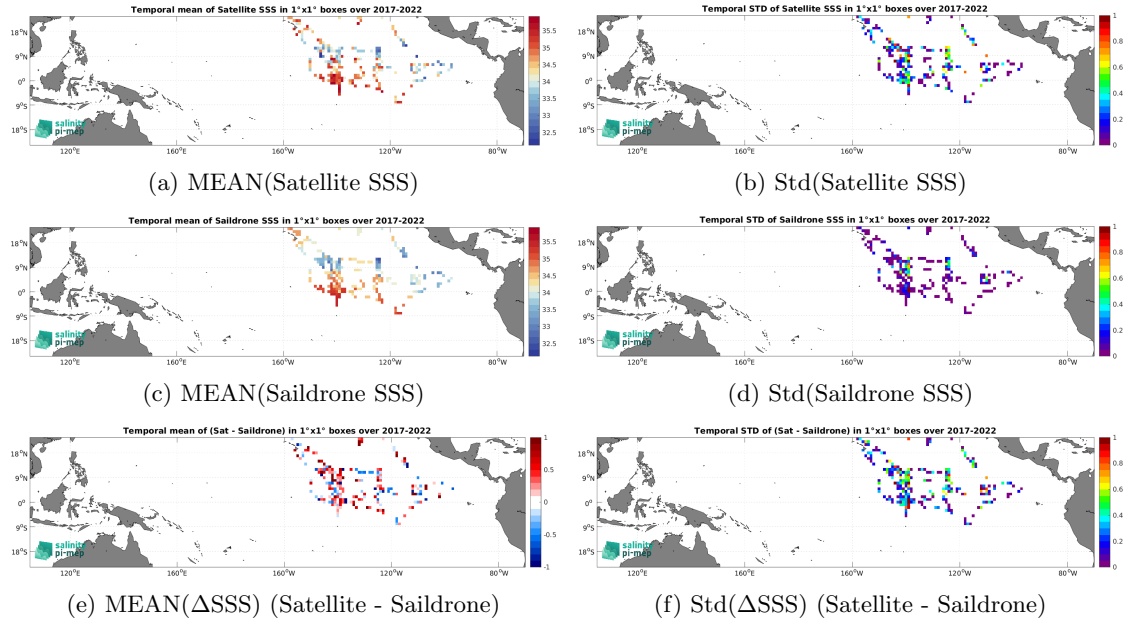
Figure 6: Temporal mean (left) and Std (right) of SSS from SMOS SSS L2Q v331 - 0.25 Deg (CATDS-CPDC) (top), Saildrone (middle), and of \Delta SSS (Satellite - Saildrone). Only match-up pairs are used to generate these maps.
