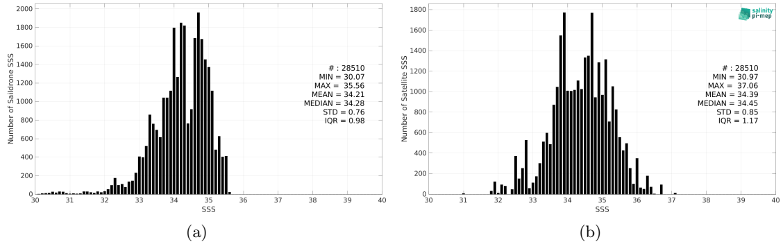
Figure 2: Histograms of SSS from Saildrone (a) and SMOS SSS L2Q v331 - 0.25 Deg (CATDS-CPDC) (b) considering all match-up pairs per bins of 0.1 over the Tropical Pacific Ocean Pi-MEP region and for the full satellite product period.
