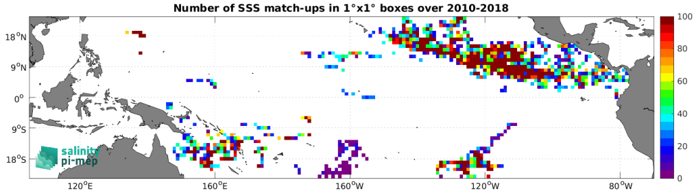
Figure 3: Number of SSS match-ups between Surface drifters SSS and the SMOS SSS L2Q v331 - 0.25 Deg (CATDS-CPDC) SSS product for the Tropical Pacific Ocean Pi-MEP region over 1^\circ \times 1^\circ boxes and for the full satellite product period.
