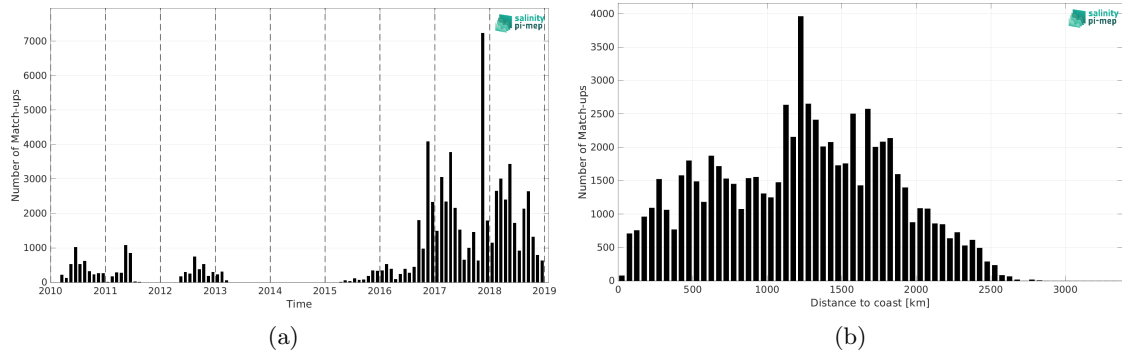
Figure 1: Number of match-ups between Surface drifters and SMOS SSS L2Q v331 - 0.25 Deg (CATDS-CPDC) SSS as a function of time (a) and as function of the distance to coast (b) over the Tropical Pacific Ocean Pi-MEP region and for the full satellite product period.
