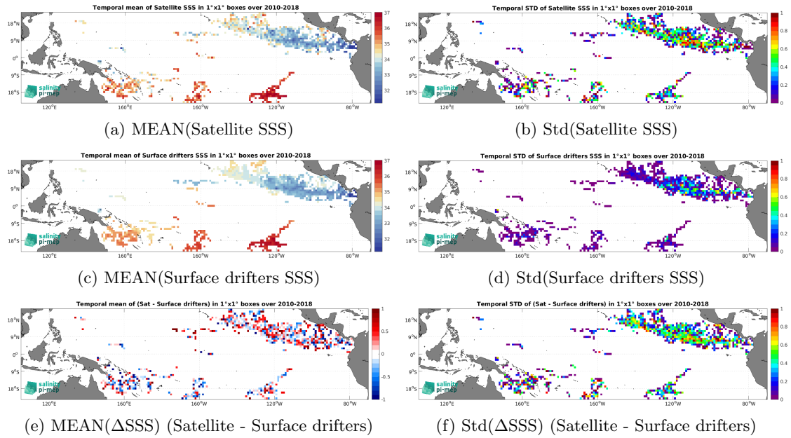
Figure 5: Temporal mean (left) and Std (right) of SSS from SMOS SSS L2Q v331 - 0.25 Deg (CATDS-CPDC) (top), Surface drifters (middle), and of \Delta SSS (Satellite - Surface drifters). Only match-up pairs are used to generate these maps.
