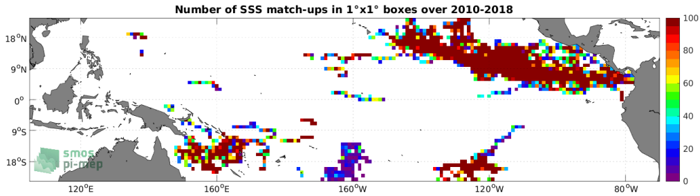
Figure 3: Number of SSS match-ups between Surface drifters SSS and the SMOS SSS L2Q v331 - 0.25 Deg (CATDS-CPDC) SSS product for the Tropical Pacific Ocean Pi-MEP region over 1^\circ \times 1^\circ boxes and for the full satellite product period.
