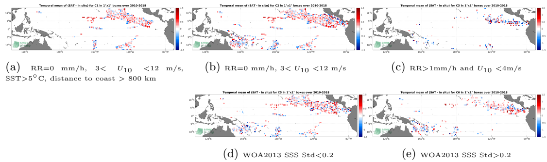
Figure 11: Temporal mean gridded over spatial boxes of size 1^\circ \times 1^\circ of \Delta\text{SSS} (SMOS SSS L2Q v331 - 0.25 Deg (CATDS-CPDC) - Surface drifters) for 5 different subdatasets corresponding to: RR=0 mm/h, 3 < U_{10} < 12 m/s, SST > 5^\circ\text{C} , distance to coast > 800 km (a), RR=0 mm/h, 3 < U_{10} < 12 m/s (b), RR > 1 mm/h and U_{10} < 4 m/s (c), WOA2013 SSS Std < 0.2 (d), WOA2013 SSS Std > 0.2 (e).
