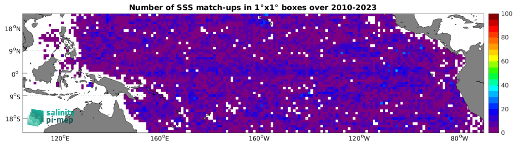
Figure 4: Number of SSS match-ups between Argo SSS and the SMOS SSS L2Q v331 - 0.25 Deg (CATDS-CPDC) SSS product for the Tropical Pacific Ocean Pi-MEP region over 1^\circ \times 1^\circ boxes and for the full satellite product period.
