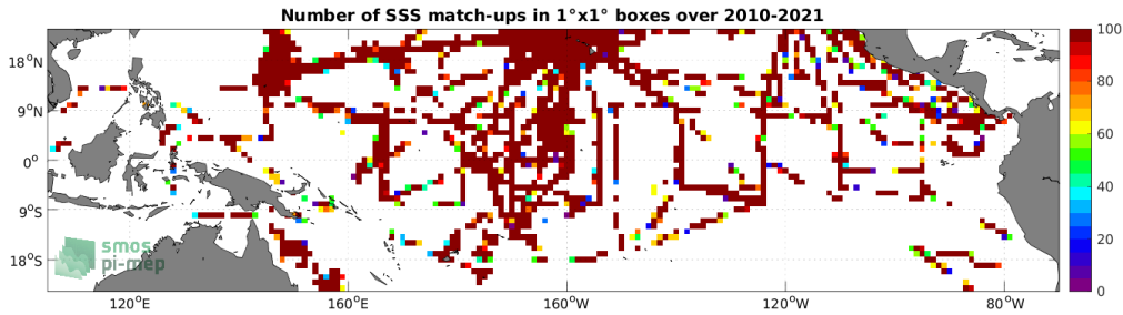
Figure 4: Number of SSS match-ups between TSG (SAMOS) SSS and the SMOS SSS L2Q v330 - 0.25 Deg (CATDS-CPDC) SSS product for the Tropical Pacific Ocean Pi-MEP region over 1^\circ \times 1^\circ boxes and for the full satellite product period.
