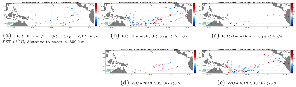
Figure 12: Temporal mean gridded over spatial boxes of size 1^{\circ}\times 1^{\circ} of \Delta SSS (SMOS SSS L2Q v330 - 0.25 Deg (CATDS-CPDC) - TSG (GOSUD-Research-vessel)) for 5 different subdatasets corresponding to:RR=0 mm/h, 3 < U_{10} < 12 m/s, SST >5^{\circ}\text{C} , distance to coast > 800 km (a), RR=0 mm/h, 3 < U_{10} < 12 m/s (b), RR >1 mm/h and U_{10} < 4 m/s (c), WOA2013 SSS Std <0.2 (d), WOA2013 SSS Std >0.2 (e).
