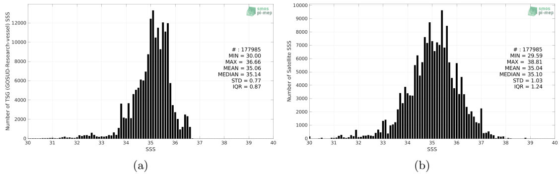
Figure 2: Histograms of SSS from TSG (GOSUD-Research-vessel) (a) and SMOS SSS L2Q v330 - 0.25 Deg (CATDS-CPDC) (b) considering all match-up pairs per bins of 0.1 over the Tropical Pacific Ocean Pi-MEP region and for the full satellite product period.
