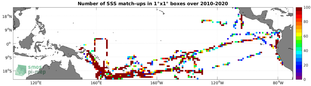
Figure 4: Number of SSS match-ups between TSG (GOSUD-Research-vessel) SSS and the SMOS SSS L2Q v330 - 0.25 Deg (CATDS-CPDC) SSS product for the Tropical Pacific Ocean Pi-MEP region over 1^\circ \times 1^\circ boxes and for the full satellite product period.
