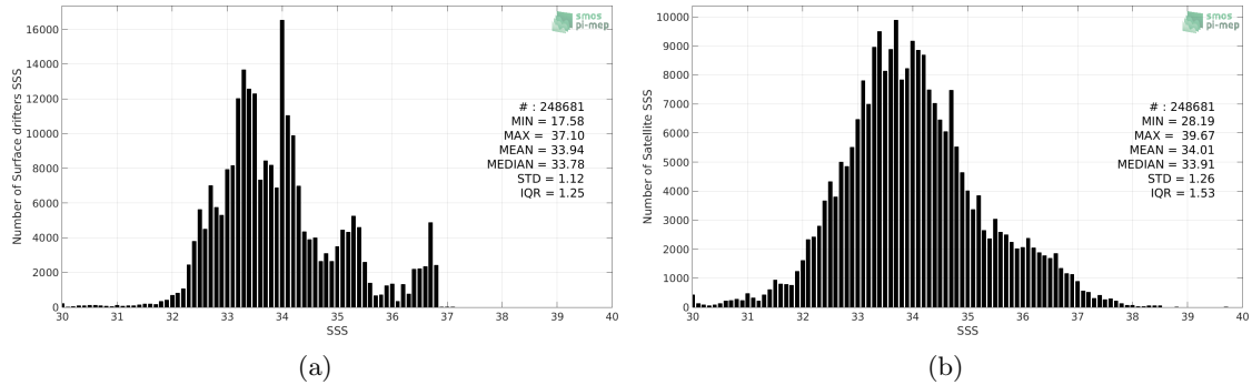
Figure 2: Histograms of SSS from Surface drifters (a) and SMOS SSS L2Q v330 - 0.25 Deg (CATDS-CPDC) (b) considering all match-up pairs per bins of 0.1 over the Tropical Pacific Ocean Pi-MEP region and for the full satellite product period.
