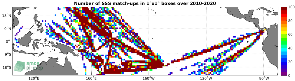
Figure 4: Number of SSS match-ups between TSG (LEGOS-DM) SSS and the SMOS SSS L2Q v321 - 0.25 Deg (CATDS-CPDC) SSS product for the Tropical Pacific Ocean Pi-MEP region over 1^\circ \times 1^\circ boxes and for the full satellite product period.
