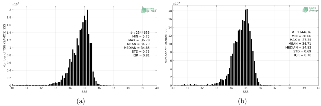
Figure 2: Histograms of SSS from TSG (SAMOS) (a) and SMOS SSS L3 v317 - Monthly - 25 km (CATDS-CPDC) (b) considering all match-up pairs per bins of 0.1 over the Tropical Pacific Ocean Pi-MEP region and for the full satellite product period.
