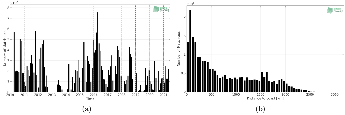
Figure 1: Number of match-ups between TSG (SAMOS) and SMOS SSS L3 v317 - Monthly - 25 km (CATDS-CPDC) SSS as a function of time (a) and as function of the distance to coast (b) over the Tropical Pacific Ocean Pi-MEP region and for the full satellite product period.
