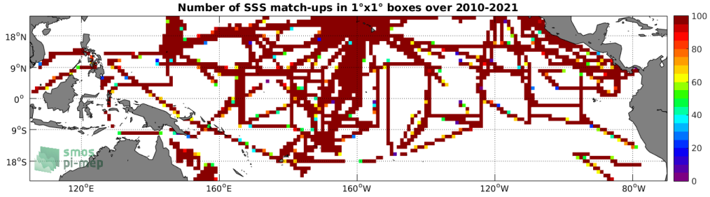
Figure 4: Number of SSS match-ups between TSG (SAMOS) SSS and the SMOS SSS L3 v317 - Monthly - 25 km (CATDS-CPDC) SSS product for the Tropical Pacific Ocean Pi-MEP region over 1^\circ \times 1^\circ boxes and for the full satellite product period.
