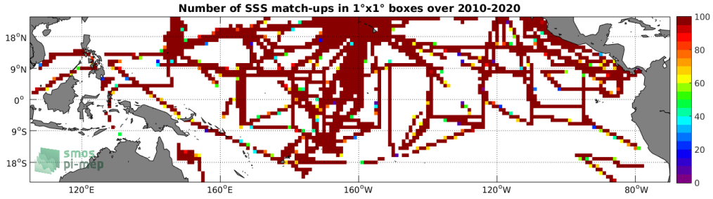
Figure 4: Number of SSS match-ups between TSG (SAMOS) SSS and the SMOS SSS L3 v317 - Monthly - 25 km (CATDS-CPDC) SSS product for the Tropical Pacific Ocean Pi-MEP region over 1^\circ \times 1^\circ boxes and for the full satellite product period.
