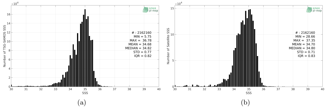
Figure 2: Histograms of SSS from TSG-SAMOS (a) and SMOS L3 v317 - Monthly - 25 km (CATDS-CPDC) (b) considering all match-up pairs per bins of 0.1 over the Tropical Pacific Ocean Pi-MEP region and for the full satellite product period.
