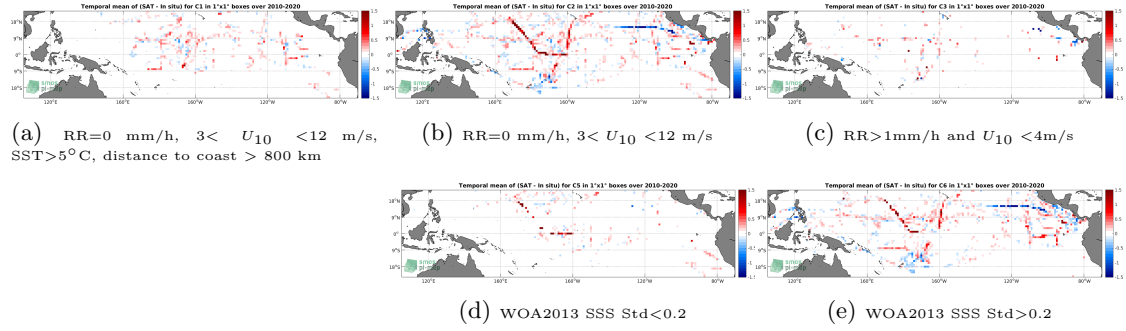
Figure 12: Temporal mean gridded over spatial boxes of size 1^\circ \times 1^\circ of \Delta SSS (SMOS L3 v317 - Monthly - 25 km (CATDS-CPDC) - TSG-SAMOS) for 5 different subdatasets corresponding to: RR=0 mm/h, 3 < U_{10} < 12 m/s, SST > 5^\circ C , distance to coast > 800 km (a), RR=0 mm/h, 3 < U_{10} < 12 m/s (b), RR > 1 mm/h and U_{10} < 4 m/s (c), WOA2013 SSS Std < 0.2 (d), WOA2013 SSS Std > 0.2 (e).
