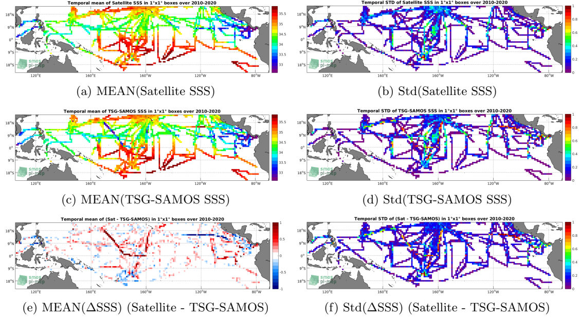
Figure 6: Temporal mean (left) and Std (right) of SSS from SMOS L3 v317 - Monthly - 25 km (CATDS-CPDC) (top), TSG-SAMOS (middle), and of \Delta SSS (Satellite - TSG-SAMOS). Only match-up pairs are used to generate these maps.
