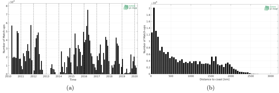
Figure 1: Number of match-ups between TSG-SAMOS and SMOS L3 v317 - Monthly - 25 km (CATDS-CPDC) SSS as a function of time (a) and as function of the distance to coast (b) over the Tropical Pacific Ocean Pi-MEP region and for the full satellite product period.
