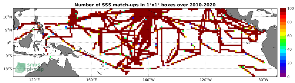
Figure 4: Number of SSS match-ups between TSG-SAMOS SSS and the SMOS L3 v317 - Monthly - 25 km (CATDS-CPDC) SSS product for the Tropical Pacific Ocean Pi-MEP region over 1°x1° boxes and for the full satellite product period.
