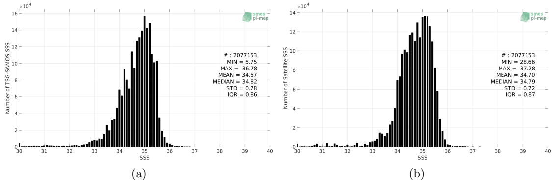
Figure 2: Histograms of SSS from TSG-SAMOS (a) and SMOS-L3-CATDS-CPDC-V317-MONTHLY-25KM (b) considering all match-up pairs per bins of 0.1 over the Tropical Pacific Ocean Pi-MEP region and for the full satellite product period.
