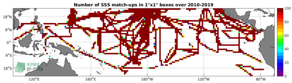
Figure 4: Number of SSS match-ups between TSG-SAMOS SSS and the SMOS-L3-CATDS-CPDC-V317-MONTHLY-25KM SSS product for the Tropical Pacific Ocean Pi-MEP region over 1°x1° boxes and for the full satellite product period.
