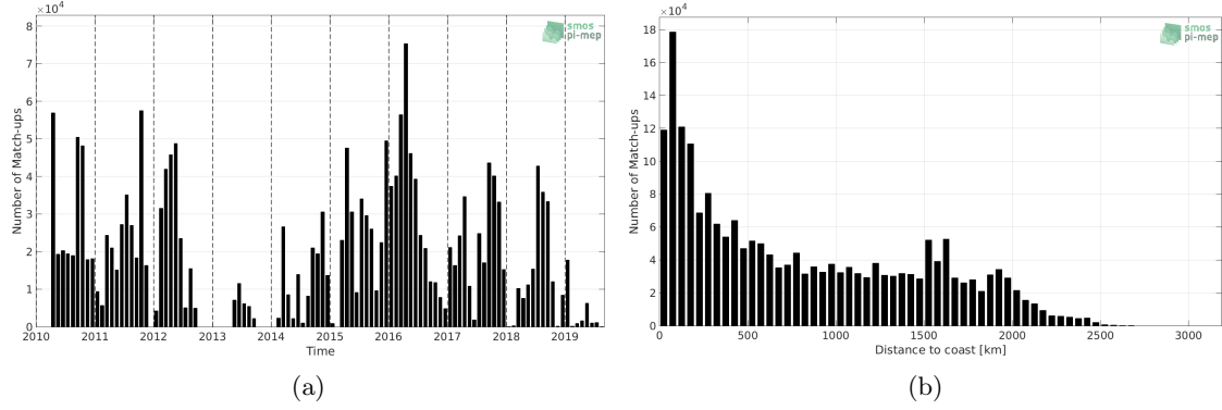
Figure 1: Number of match-ups between TSG-SAMOS and SMOS-L3-CATDS-CPDC-V317-MONTHLY-25KM SSS as a function of time (a) and as function of the distance to coast (b) over the Tropical Pacific Ocean Pi-MEP region and for the full satellite product period.
