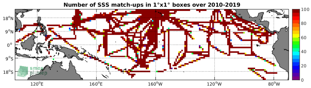
Figure 4: Number of SSS match-ups between TSG-SAMOS SSS and the SMOS-L3-CATDS-CPDC-V317-MONTHLY-25KM SSS product for the Tropical Pacific Ocean Pi-MEP region over 1^\circ \times 1^\circ boxes and for the full satellite product period.
