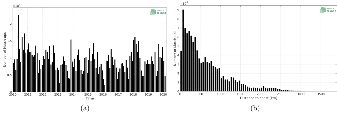
Figure 1: Number of match-ups between TSG (LEGOS-DM) and SMOS SSS L3 v317 - Monthly - 25 km (CATDS-CPDC) SSS as a function of time (a) and as function of the distance to the coast (b) over the Tropical Pacific Ocean Pi-MEP region and for the full satellite product period.
