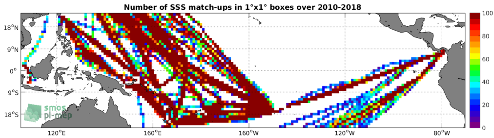
Figure 4: Number of SSS match-ups between TSG-LEGOS-DM SSS and the SMOS-L3-CATDS-CPDC-V317-MONTHLY-25KM SSS product for the Tropical Pacific Ocean Pi-MEP region over 1°x1° boxes and for the full satellite product period.
