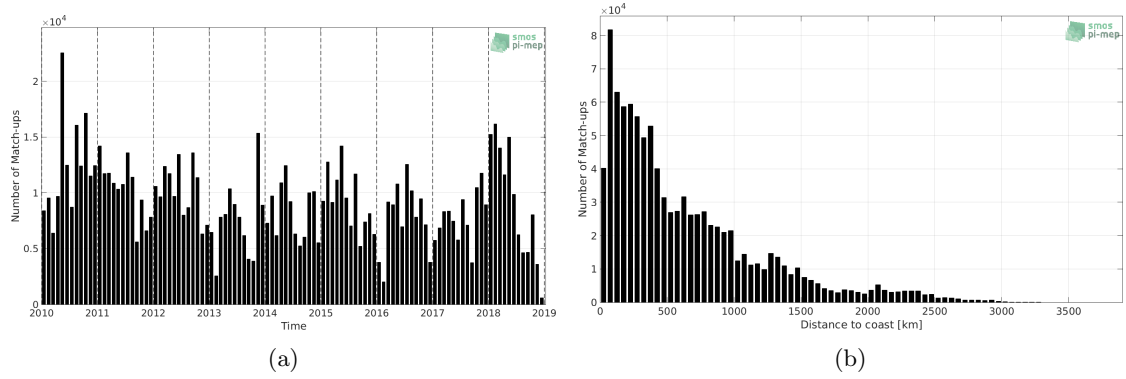
Figure 1: Number of match-ups between TSG-LEGOS-DM and SMOS-L3-CATDS-CPDC-V317-MONTHLY-25KM SSS as a function of time (a) and as function of the distance to coast (b) over the Tropical Pacific Ocean Pi-MEP region and for the full satellite product period.
