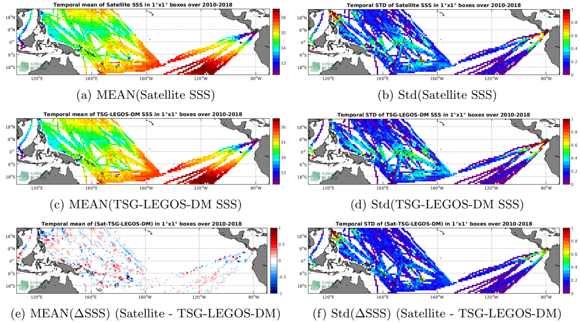
Figure 6: Temporal mean (left) and Std (right) of SSS from SMOS-L3-CATDS-CPDC-V317-MONTHLY-25KM (top), TSG-LEGOS-DM (middle), and of \Delta SSS (Satellite - TSG-LEGOS-DM). Only match-up pairs are used to generate these maps.
