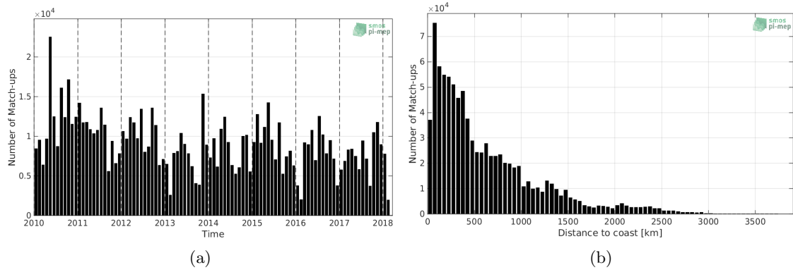
Figure 1: Number of match-ups between TSG-LEGOS-DM and SMOS-L3-CATDS-CPDC-V317-MONTHLY-25KM SSS as a function of time (a) and as function of the distance to coast (b) over the Tropical Pacific Ocean Pi-MEP region and for the full satellite product period.
