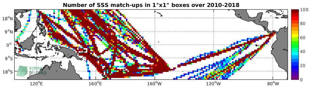
Figure 4: Number of SSS match-ups between TSG-LEGOS-DM SSS and the SMOS-L3-CATDS-CPDC-V317-MONTHLY-25KM SSS product for the Tropical Pacific Ocean Pi-MEP region over 1^{\circ} \times 1^{\circ} boxes and for the full satellite product period.
