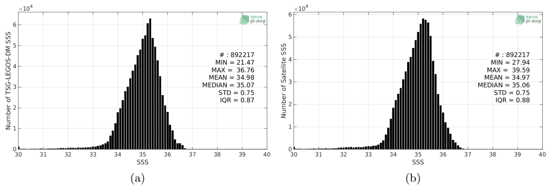
Figure 2: Histograms of SSS from TSG-LEGOS-DM (a) and SMOS-L3-CATDS-CPDC-V317-MONTHLY-25KM (b) considering all match-up pairs per bins of 0.1 over the Tropical Pacific Ocean Pi-MEP region and for the full satellite product period.
