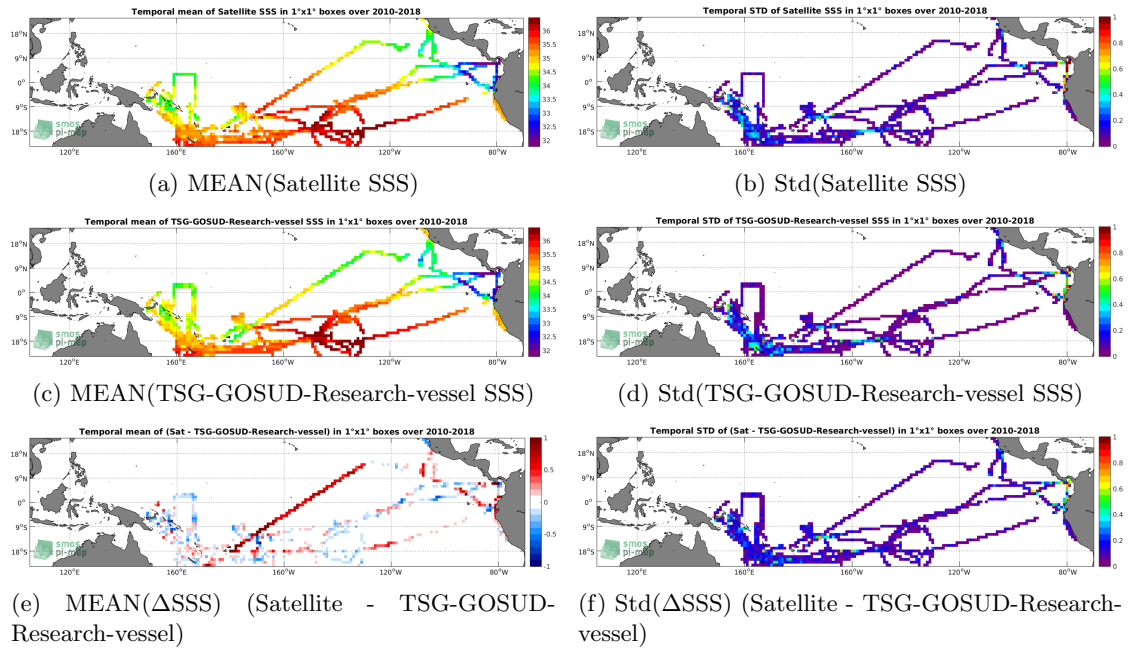
Figure 6: Temporal mean (left) and Std (right) of SSS from SMOS L3 v317 - Monthly - 25 km (CATDS-CPDC) (top), TSG-GOSUD-Research-vessel (middle), and of \Delta SSS (Satellite - TSG-GOSUD-Research-vessel). Only match-up pairs are used to generate these maps.
