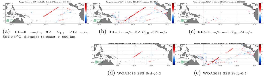
Figure 12: Temporal mean gridded over spatial boxes of size 1^{\circ}\times 1^{\circ} of \Delta SSS (SMOS L3 v317 - Monthly - 25 km (CATDS-CPDC) - TSG-GOSUD-Research-vessel) for 5 different subdatasets corresponding to:RR=0 mm/h, 3 < U_{10} < 12 m/s, SST >5^{\circ}\text{C} , distance to coast > 800 km (a), RR=0 mm/h, 3 < U_{10} < 12 m/s (b), RR >1 mm/h and U_{10} < 4 m/s (c), WOA2013 SSS Std <0.2 (d), WOA2013 SSS Std >0.2 (e).
