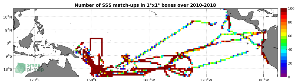
Figure 4: Number of SSS match-ups between TSG-GOSUD-Research-vessel SSS and the SMOS L3 v317 - Monthly - 25 km (CATDS-CPDC) SSS product for the Tropical Pacific Ocean Pi-MEP region over 1°x1° boxes and for the full satellite product period.
