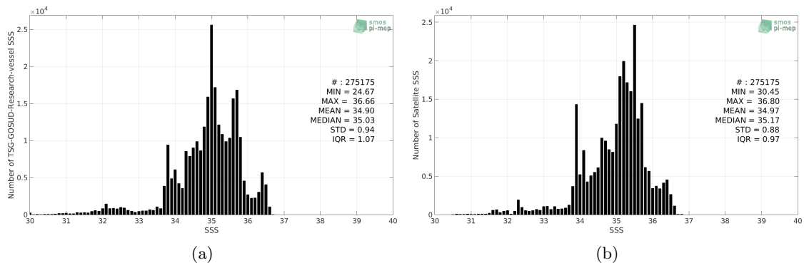
Figure 2: Histograms of SSS from TSG-GOSUD-Research-vessel (a) and SMOS L3 v317 - Monthly - 25 km (CATDS-CPDC) (b) considering all match-up pairs per bins of 0.1 over the Tropical Pacific Ocean Pi-MEP region and for the full satellite product period.
