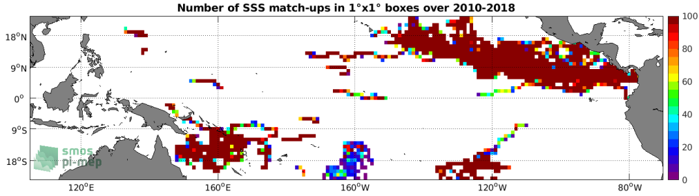
Figure 3: Number of SSS match-ups between Surface drifters SSS and the SMOS SSS L3 v317 - Monthly - 25 km (CATDS-CPDC) SSS product for the Tropical Pacific Ocean Pi-MEP region over 1^\circ \times 1^\circ boxes and for the full satellite product period.
