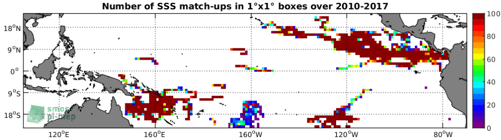
Figure 3: Number of SSS match-ups between Surface drifters SSS and the SMOS-L3-CATDS-CPDC-V317-MONTHLY-25KM SSS product for the Tropical Pacific Ocean Pi-MEP region over 1^\circ \times 1^\circ boxes and for the full satellite product period.
