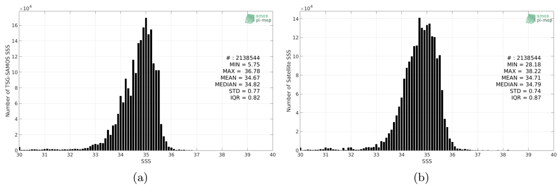
Figure 2: Histograms of SSS from TSG-SAMOS (a) and SMOS L3 v317 - 10 Days - 25 km (CATDS-CPDC) (b) considering all match-up pairs per bins of 0.1 over the Tropical Pacific Ocean Pi-MEP region and for the full satellite product period.
