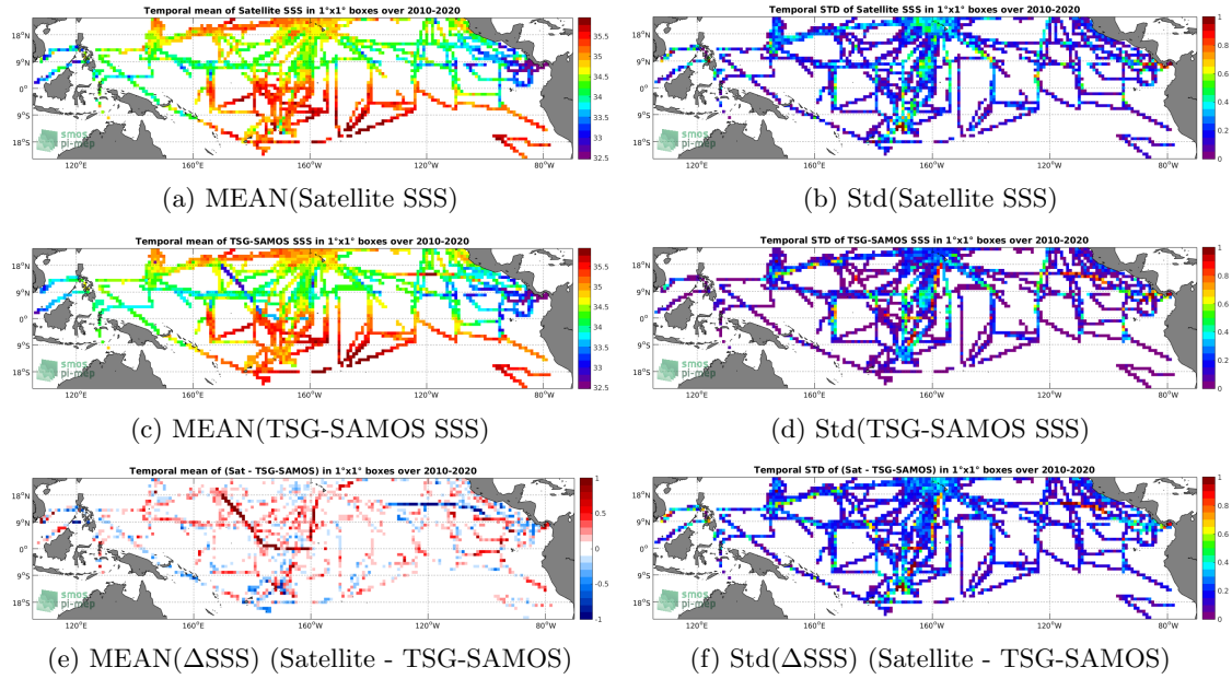
Figure 6: Temporal mean (left) and Std (right) of SSS from SMOS L3 v317 - 10 Days - 25 km (CATDS-CPDC) (top), TSG-SAMOS (middle), and of \Delta SSS (Satellite - TSG-SAMOS). Only match-up pairs are used to generate these maps.
