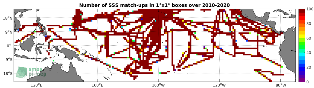
Figure 4: Number of SSS match-ups between TSG-SAMOS SSS and the SMOS L3 v317 - 10 Days - 25 km (CATDS-CPDC) SSS product for the Tropical Pacific Ocean Pi-MEP region over 1^\circ \times 1^\circ boxes and for the full satellite product period.
