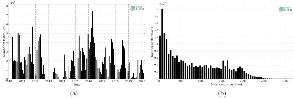
Figure 1: Number of match-ups between TSG-SAMOS and SMOS L3 v317 - 10 Days - 25 km (CATDS-CPDC) SSS as a function of time (a) and as function of the distance to coast (b) over the Tropical Pacific Ocean Pi-MEP region and for the full satellite product period.
