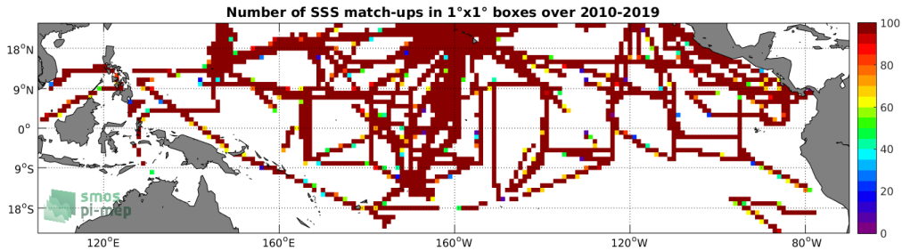
Figure 4: Number of SSS match-ups between TSG-SAMOS SSS and the SMOS-L3-CATDS-CPDC-V317-10DAYS-25KM SSS product for the Tropical Pacific Ocean Pi-MEP region over 1^\circ \times 1^\circ boxes and for the full satellite product period.
