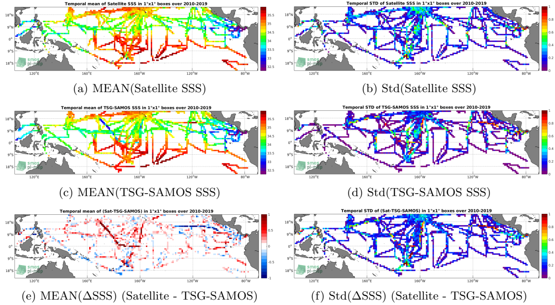
Figure 6: Temporal mean (left) and Std (right) of SSS from SMOS-L3-CATDS-CPDC-V317-10DAYS-25KM (top), TSG-SAMOS (middle), and of \Delta SSS (Satellite - TSG-SAMOS). Only match-up pairs are used to generate these maps.
