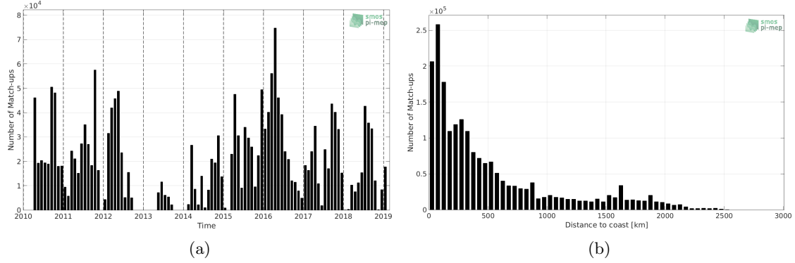
Figure 1: Number of match-ups between TSG-SAMOS and SMOS-L3-CATDS-CPDC-V317-10DAYS-25KM SSS as a function of time (a) and as function of the distance to coast (b) over the Tropical Pacific Ocean Pi-MEP region and for the full satellite product period.
