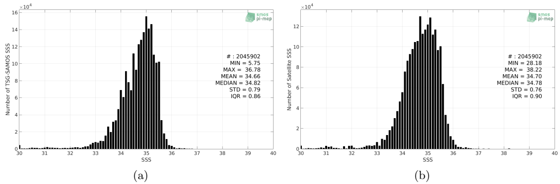
Figure 2: Histograms of SSS from TSG-SAMOS (a) and SMOS-L3-CATDS-CPDC-V317-10DAYS-25KM (b) considering all match-up pairs per bins of 0.1 over the Tropical Pacific Ocean Pi-MEP region and for the full satellite product period.
