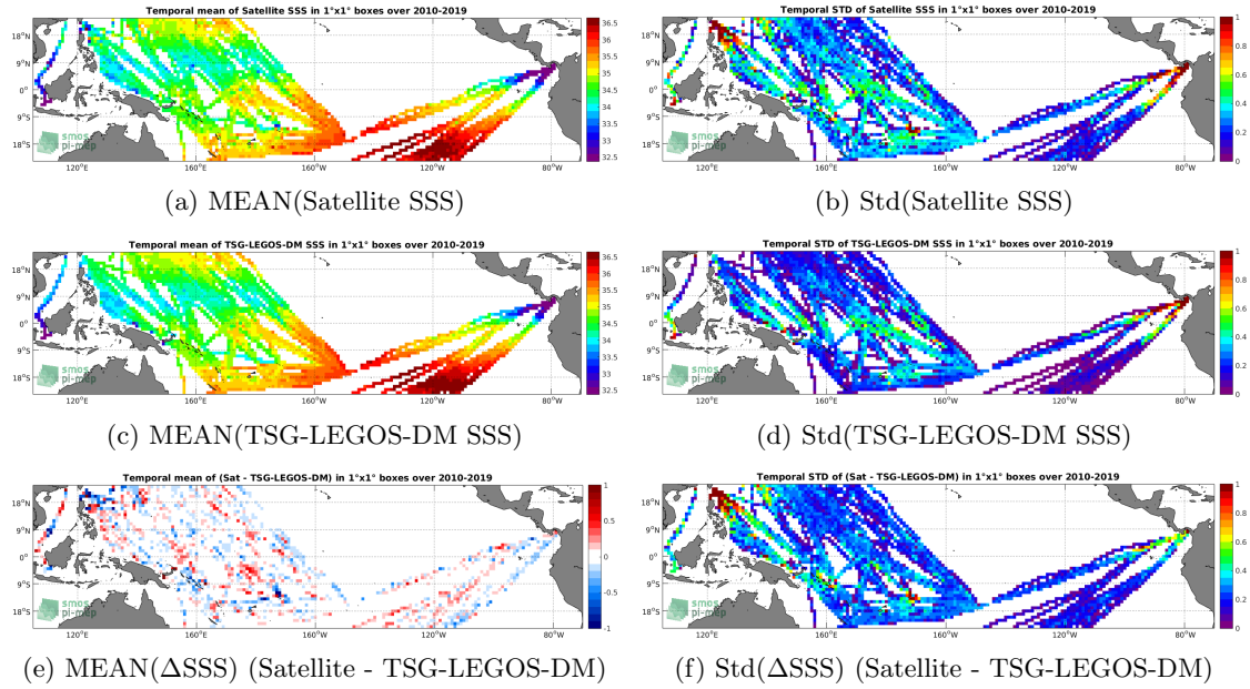
Figure 6: Temporal mean (left) and Std (right) of SSS from SMOS L3 v317 - 10 Days - 25 km (CATDS-CPDC) (top), TSG-LEGOS-DM (middle), and of \Delta SSS (Satellite - TSG-LEGOS-DM). Only match-up pairs are used to generate these maps.
