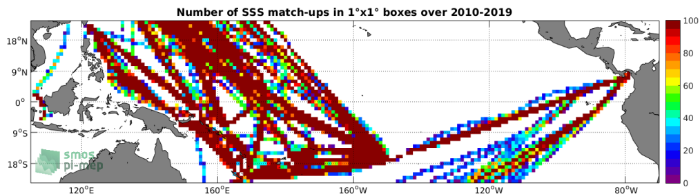
Figure 4: Number of SSS match-ups between TSG-LEGOS-DM SSS and the SMOS L3 v317 - 10 Days - 25 km (CATDS-CPDC) SSS product for the Tropical Pacific Ocean Pi-MEP region over 1^\circ \times 1^\circ boxes and for the full satellite product period.
