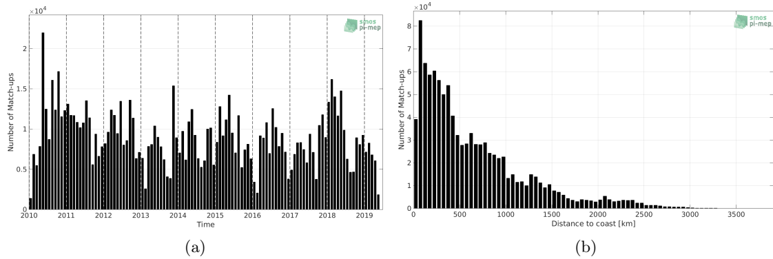
Figure 1: Number of match-ups between TSG-LEGOS-DM and SMOS L3 v317 - 10 Days - 25 km (CATDS-CPDC) SSS as a function of time (a) and as function of the distance to coast (b) over the Tropical Pacific Ocean Pi-MEP region and for the full satellite product period.
