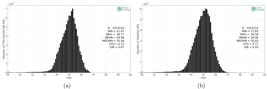
Figure 2: Histograms of SSS from TSG-LEGOS-DM (a) and SMOS L3 v317 - 10 Days - 25 km (CATDS-CPDC) (b) considering all match-up pairs per bins of 0.1 over the Tropical Pacific Ocean Pi-MEP region and for the full satellite product period.
