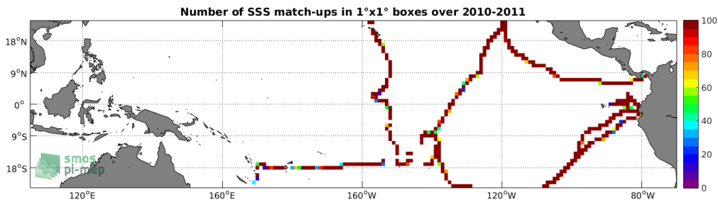
Figure 4: Number of SSS match-ups between TSG (GOSUD-Sailing-ship) SSS and the SMOS SSS L3 v317 - 10 Days - 25 km (CATDS-CPDC) SSS product for the Tropical Pacific Ocean Pi-MEP region over 1^\circ \times 1^\circ boxes and for the full satellite product period.
