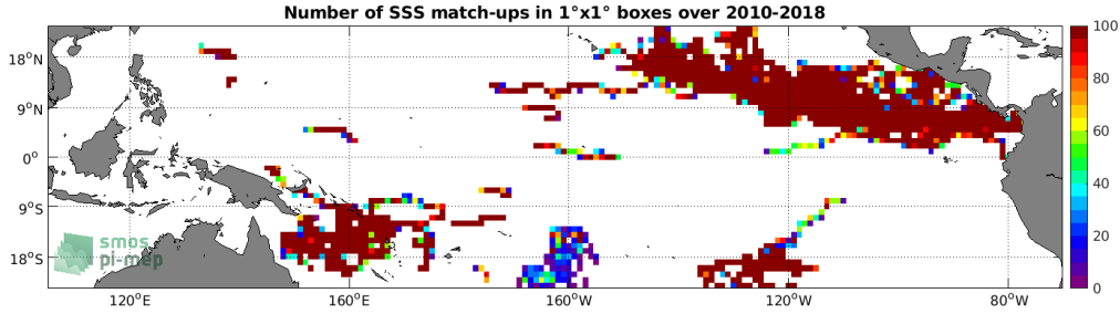
Figure 3: Number of SSS match-ups between Surface drifters SSS and the SMOS SSS L3 v317 - 10 Days - 25 km (CATDS-CPDC) SSS product for the Tropical Pacific Ocean Pi-MEP region over 1^\circ \times 1^\circ boxes and for the full satellite product period.
