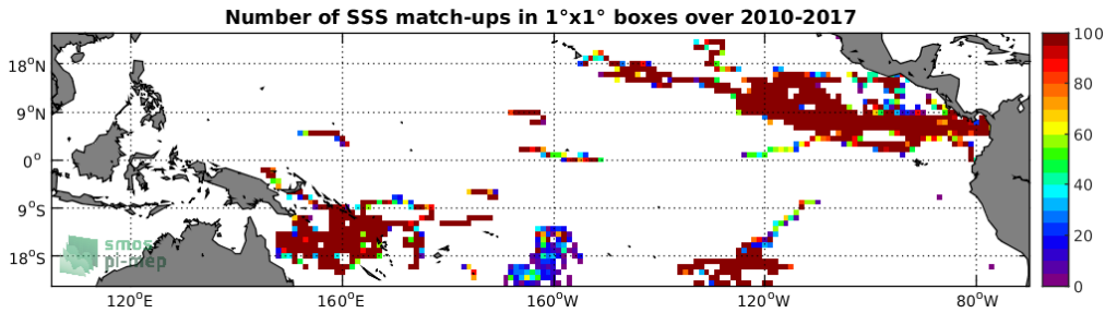
Figure 3: Number of SSS match-ups between Surface drifters SSS and the SMOS-L3-CATDS-CPDC-V317-10DAYS-25KM SSS product for the Tropical Pacific Ocean Pi-MEP region over 1^\circ \times 1^\circ boxes and for the full satellite product period.
