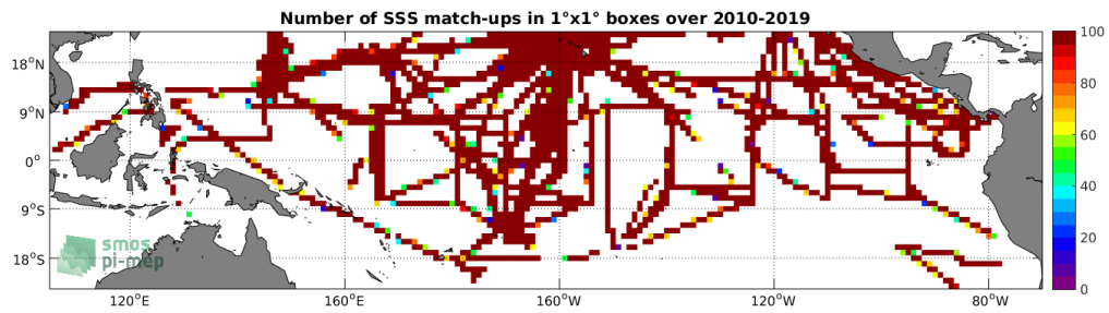
Figure 4: Number of SSS match-ups between TSG-SAMOS SSS and the SMOS-L3-CATDS-CPDC-V3-MONTHLY-25KM SSS product for the Tropical Pacific Ocean Pi-MEP region over 1°x1° boxes and for the full satellite product period.
