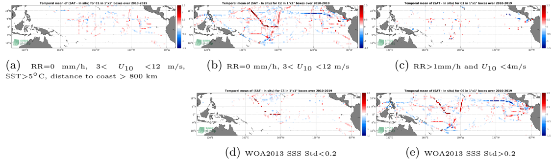
Figure 12: Temporal mean gridded over spatial boxes of size 1^\circ \times 1^\circ of \Delta SSS (SMOS-L3-CATDS-CPDC-V3-MONTHLY-25KM - TSG-SAMOS) for 5 different subdatasets corresponding to: RR=0 mm/h, 3 < U_{10} < 12 m/s, SST > 5^\circ C , distance to coast > 800 km (a), RR=0 mm/h, 3 < U_{10} < 12 m/s (b), RR > 1 mm/h and U_{10} < 4 m/s (c), WOA2013 SSS Std < 0.2 (d), WOA2013 SSS Std > 0.2 (e).
