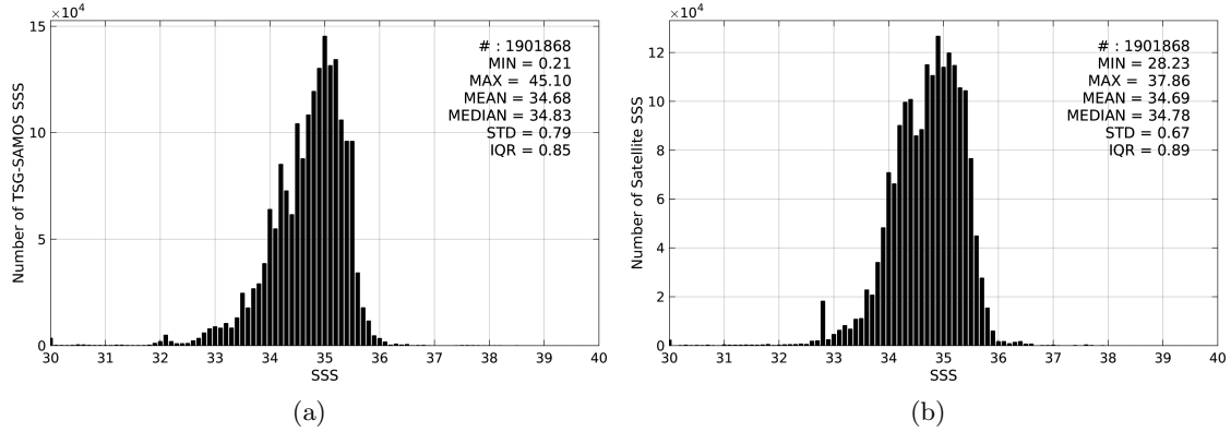
Figure 2: Histograms of SSS from TSG-SAMOS (a) and SMOS-L3-CATDS-CPDC-V3-MONTHLY-25KM (b) considering all match-up pairs per bins of 0.1 over the Tropical Pacific Ocean Pi-MEP region and for the full satellite product period.
