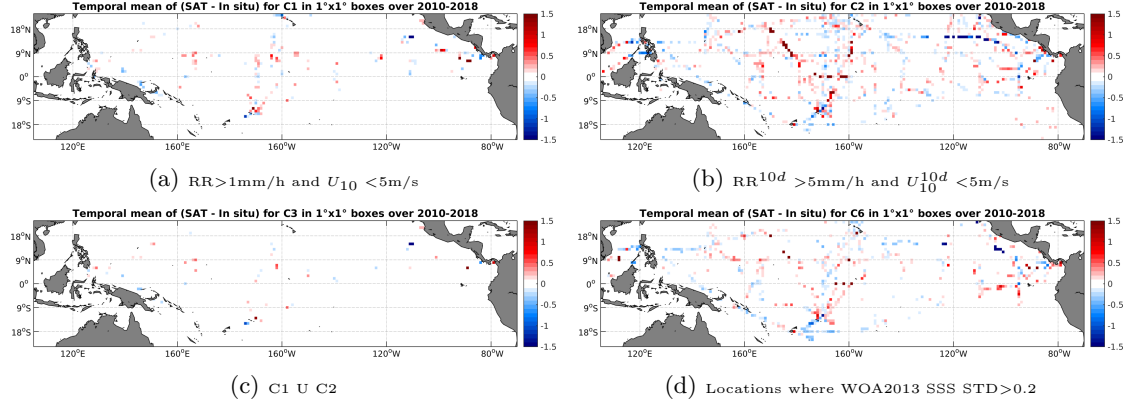
Figure 12: Temporal mean gridded over spatial boxes of size 1^\circ \times 1^\circ of \Delta SSS (SMOS-L3-CATDS-CPDC-V3-MONTHLY-25KM - TSG-SAMOS) for 4 different subdatasets corresponding to: RR > 1 mm/h and U_{10} < 5 m/s (a), RR 10d > 5 mm/h and U_{10}^{10d} < 5 m/s (b), C1 U C2 (c), Locations where WOA2013 SSS STD > 0.2 (d).
