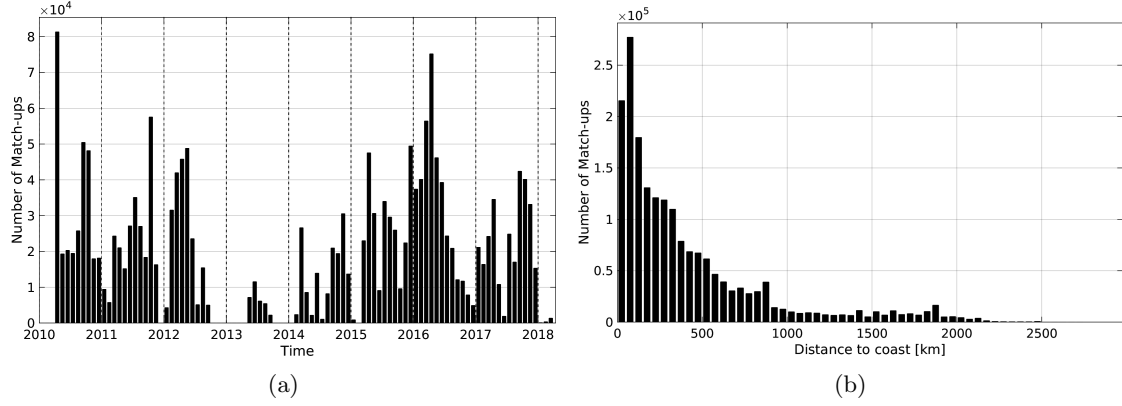
Figure 1: Number of match-ups between TSG-SAMOS and SMOS-L3-CATDS-CPDC-V3-MONTHLY-25KM SSS as a function of time (a) and as function of the distance to coast (b) over the Tropical Pacific Ocean Pi-MEP region and for the full satellite product period.
