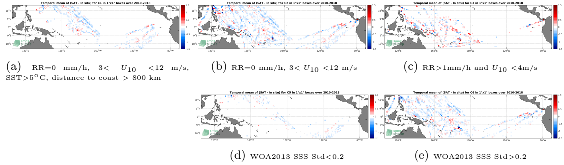
Figure 12: Temporal mean gridded over spatial boxes of size 1^\circ \times 1^\circ of \Delta SSS (SMOS-L3-CATDS-CPDC-V3-MONTHLY-25KM - TSG-LEGOS-DM) for 5 different subdatasets corresponding to: RR=0 mm/h, 3 < U_{10} < 12 m/s, SST > 5^\circ C , distance to coast > 800 km (a), RR=0 mm/h, 3 < U_{10} < 12 m/s (b), RR > 1 mm/h and U_{10} < 4 m/s (c), WOA2013 SSS Std < 0.2 (d), WOA2013 SSS Std > 0.2 (e).
