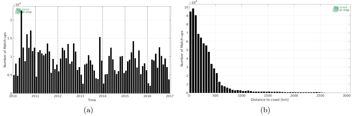
Figure 1: Number of match-ups between TSG-LEGOS-DM and SMOS-L3-CATDS-CPDC-V3-MONTHLY-25KM SSS as a function of time (a) and as function of the distance to coast (b) over the Tropical Pacific Ocean Pi-MEP region and for the full satellite product period.
