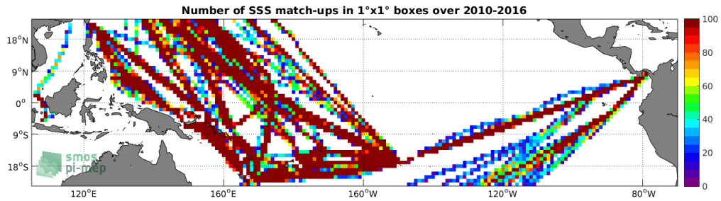
Figure 4: Number of SSS match-ups between TSG-LEGOS-DM SSS and the SMOS-L3-CATDS-CPDC-V3-MONTHLY-25KM SSS product for the Tropical Pacific Ocean Pi-MEP region over 1^\circ \times 1^\circ boxes and for the full satellite product period.
