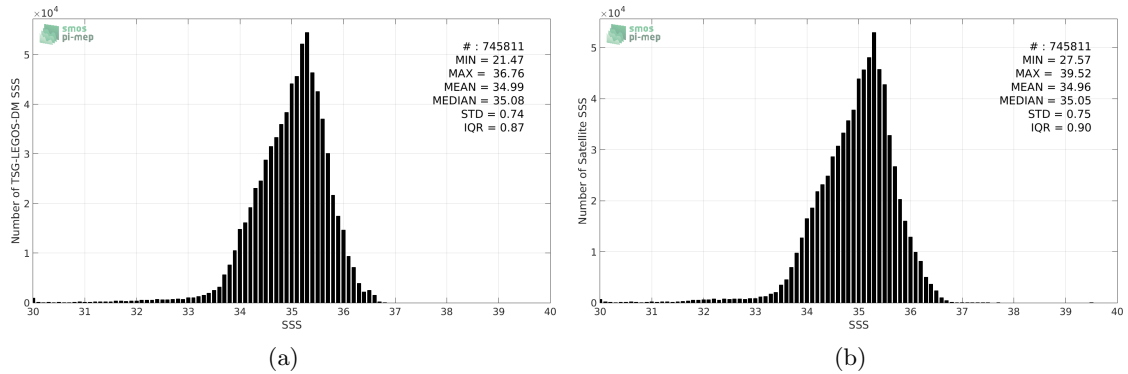
Figure 2: Histograms of SSS from TSG-LEGOS-DM (a) and SMOS-L3-CATDS-CPDC-V3-MONTHLY-25KM (b) considering all match-up pairs per bins of 0.1 over the Tropical Pacific Ocean Pi-MEP region and for the full satellite product period.
